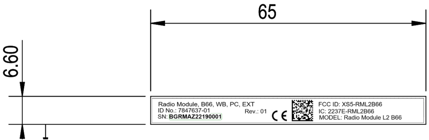
Accreditation Label dimension (text as example)
