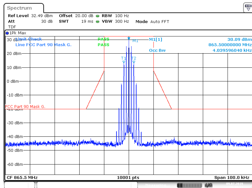
Output Signal
