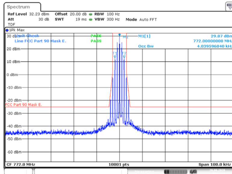
Output Signal
