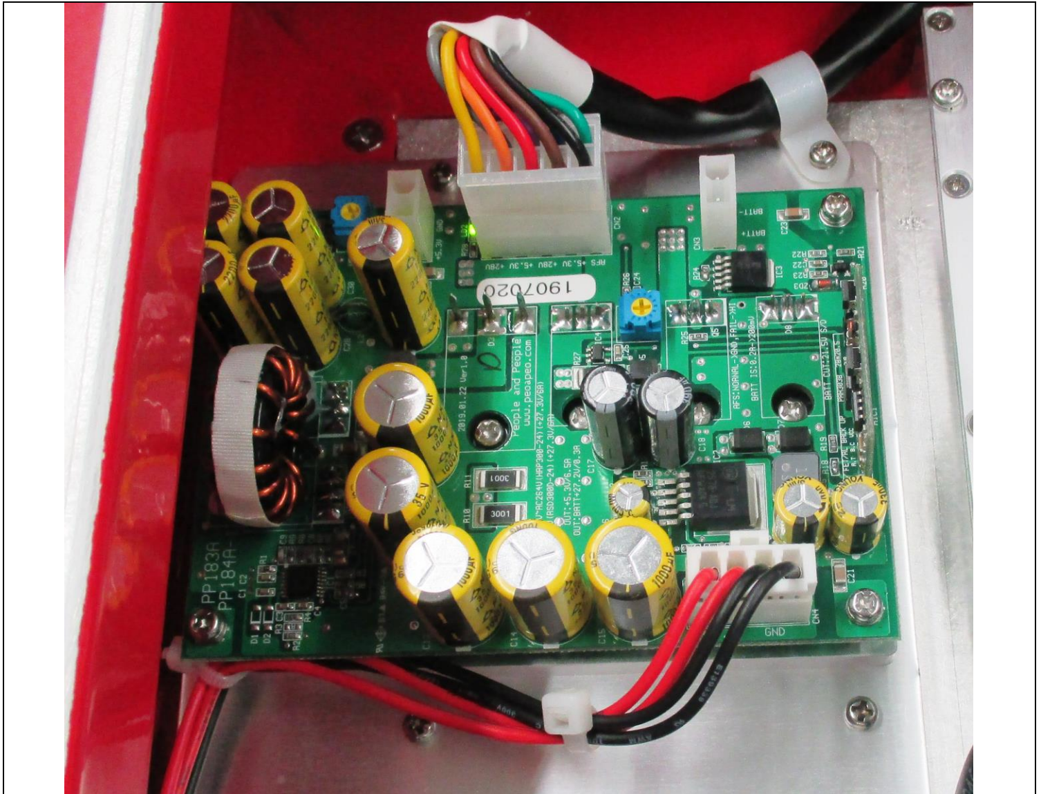
DC-DC Converter
