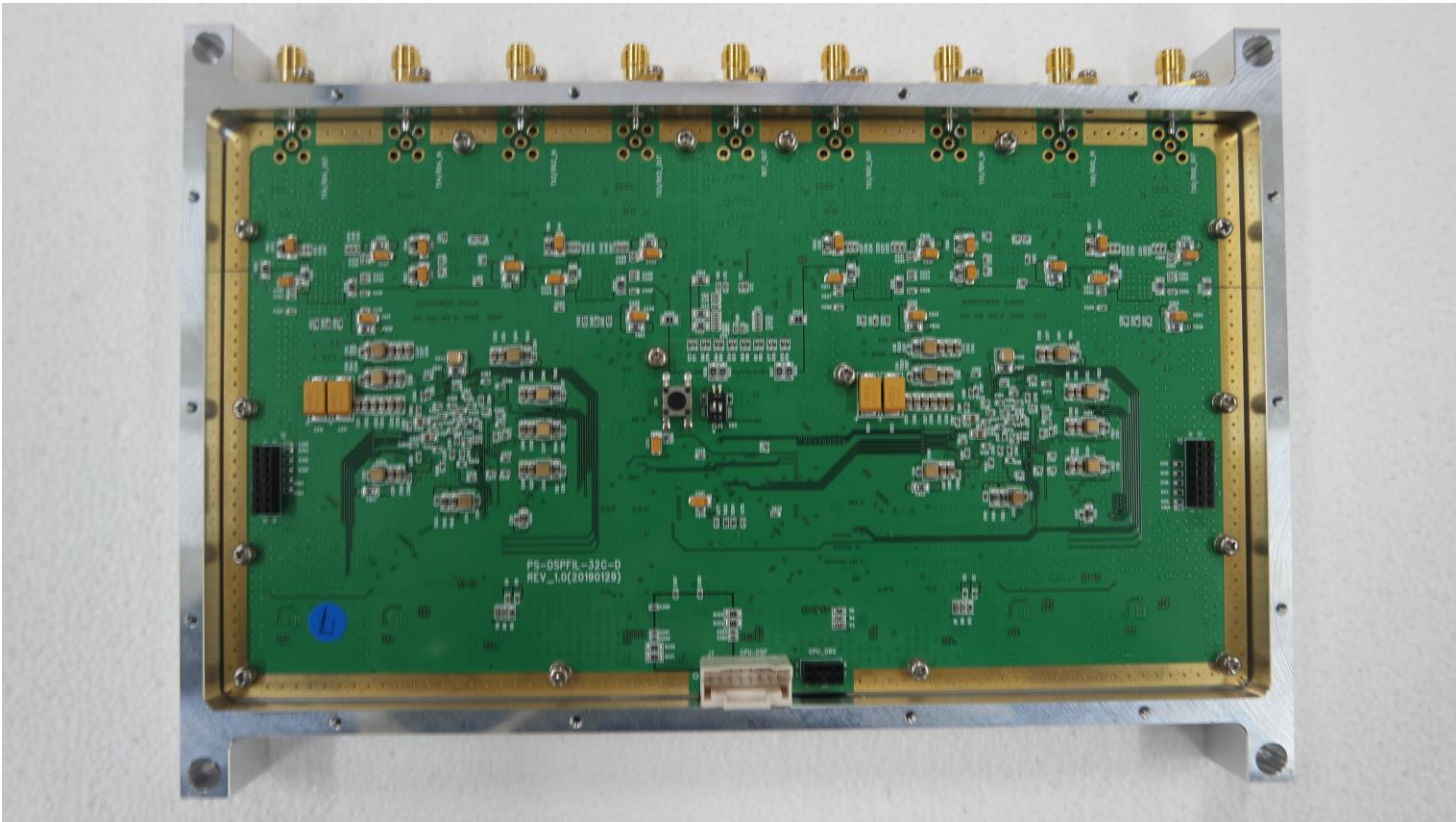
DSP Board
