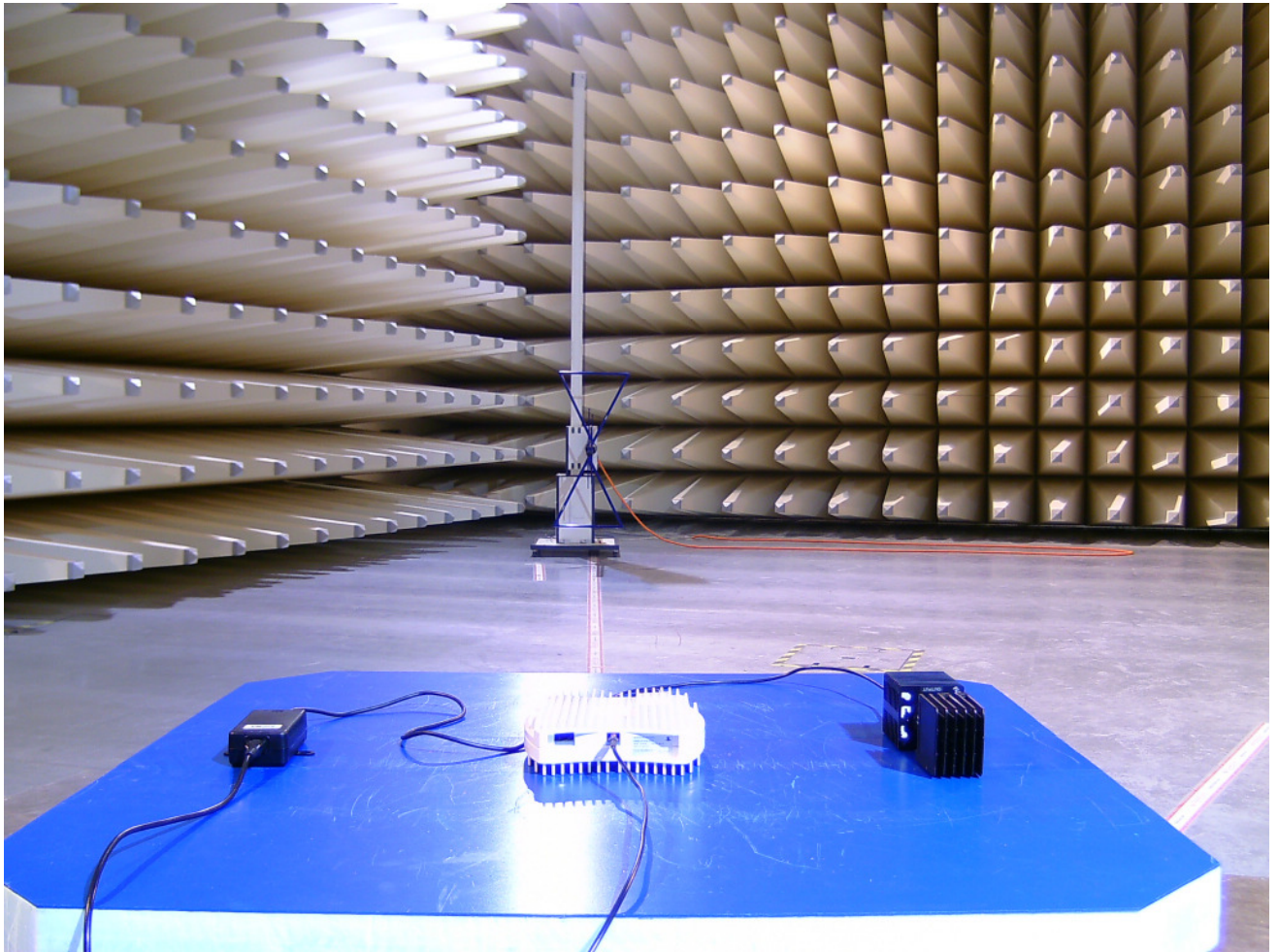
picture 8.2: Test setup: Field Strength Emission <math><1\text{ GHz}</math> @10m in the SAC
