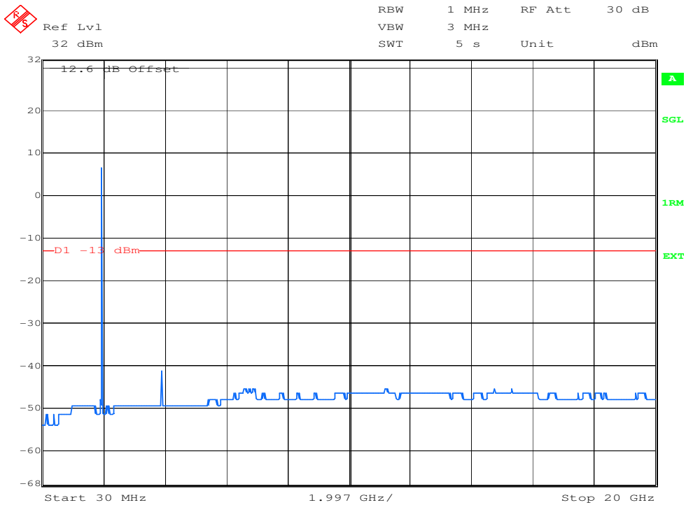
Date: 25.FEB.2010 16:02:28 plot 7.3.1.6-#1 Spurious Emissions at Antenna Terminals: §24.238, §2.1051; RSS-132, RSS-GEN; Test results; Downlink; W-CDMA > 1MHz to band edge;
