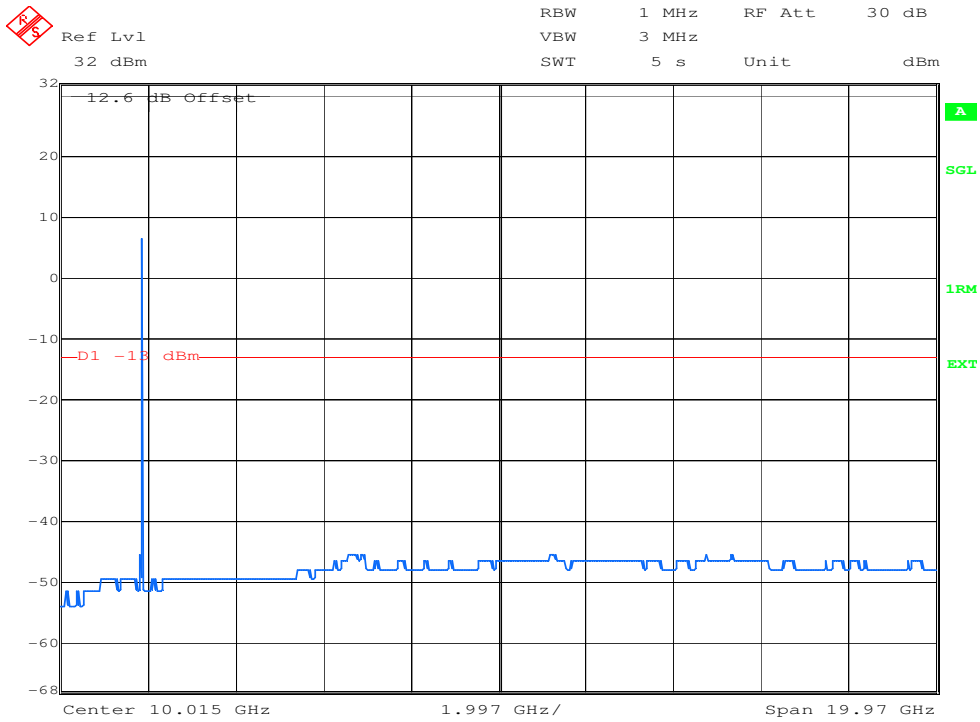
Date: 25.FEB.2010 16:10:51 plot 7.3.2.7-#1 Spurious Emissions at Antenna Terminals: §24.238, §2.1051; RSS-132, RSS-GEN; Test results; Uplink; GSM > 1MHz to band edge;
