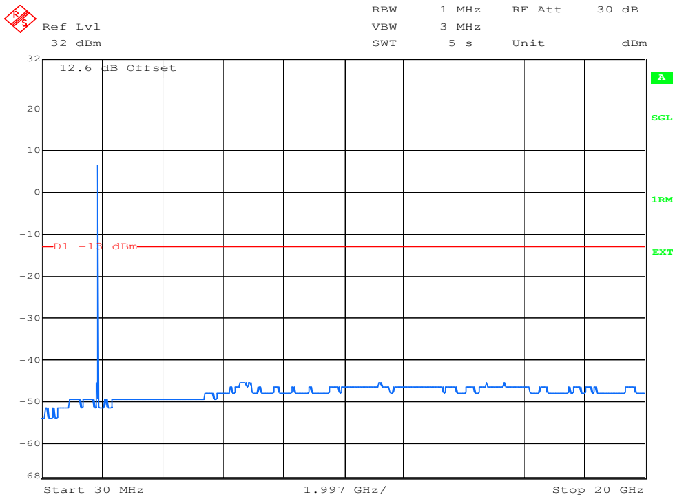
Date: 25.FEB.2010 15:43:57 plot 7.3.2.8-#1 Spurious Emissions at Antenna Terminals: §24.238, §2.1051; RSS-132, RSS-GEN; Test results; Uplink; GSM-EDGE > 1MHz to band edge;
