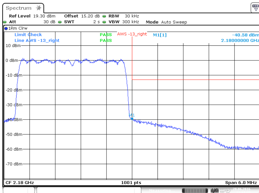
plot 7.3.3.1-#2 Intermodulation: §27.53, §2.1051; Test results; Downlink; CDMA Upper Band Edge
