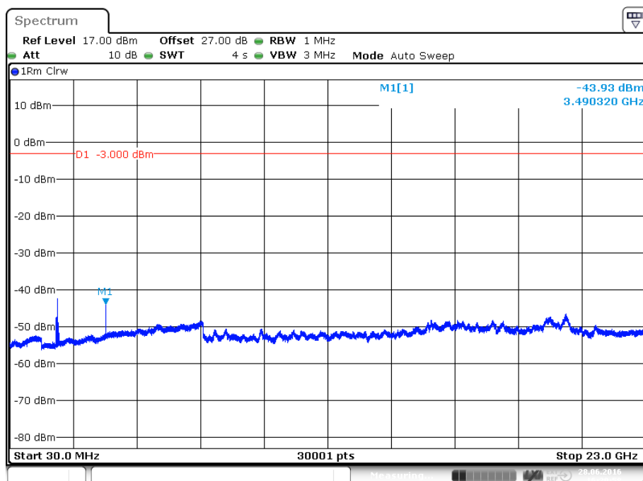
plot 6.3.4.2-#1 Spurious Emissions at Antenna Terminals: §27.53, §2.1051; Test results; Uplink; W-CDMA; carrier (1745MHz) notched
