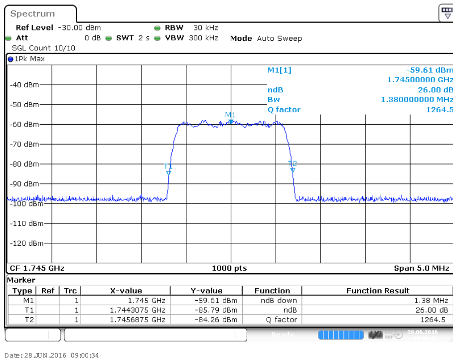
plot 5.3.6.1-#2 Occupied Bandwidth: §2.1049; Test results; 26dB Bandwidth; CDMA Input
