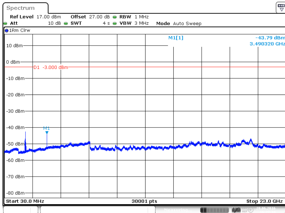
plot 6.3.4.1-#1 Spurious Emissions at Antenna Terminals: §27.53, §2.1051; Test results; Uplink; CDMA; carrier (1745MHz) notched
