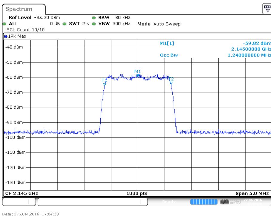
plot 5.3.3.1-#2 Occupied Bandwidth: §2.1049; Test results; Downlink; CDMA Input
