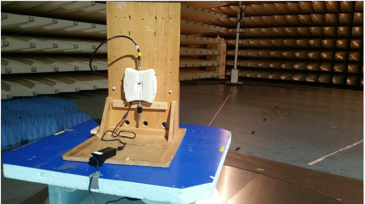
Test setup: Field Strength Emission 30 M – 1 GHz @10m in the SAC
