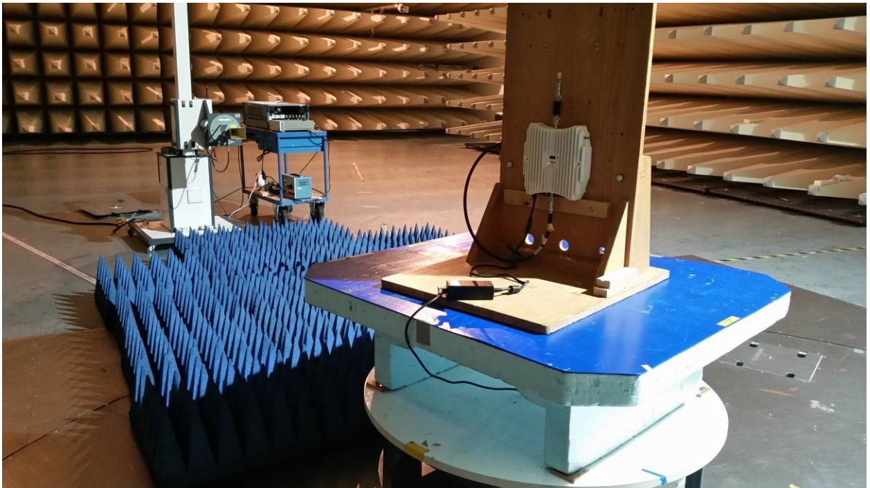
Test setup: Field Strength Emission 18 – 26.5 GHz @3m in the SAC
