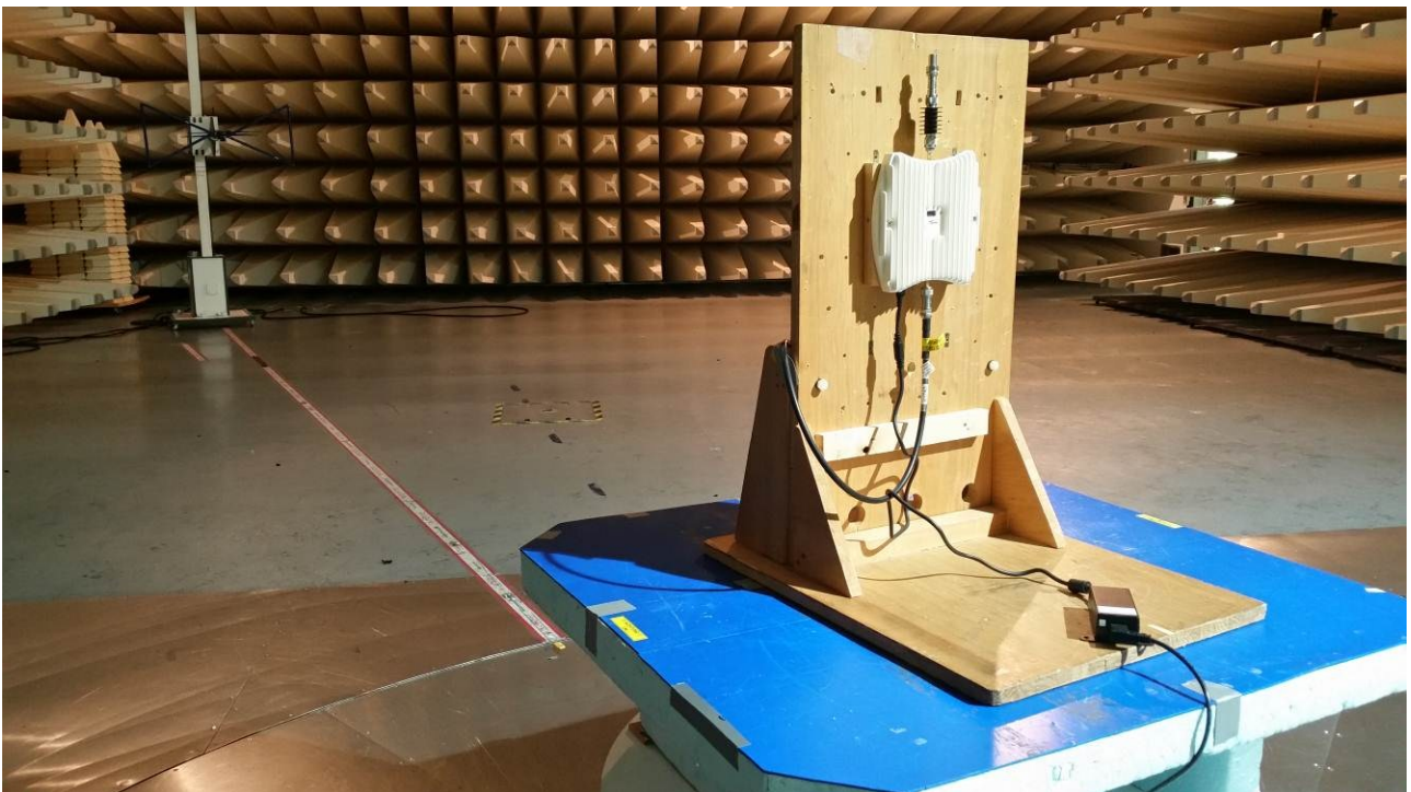
picture 8.2: Test setup: Field Strength Emission 30 M – 1 GHz @10m in the SAC
