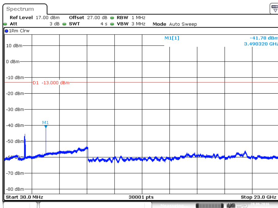
plot 6.3.4.2-#1 Spurious Emissions at Antenna Terminals: §27.53, §2.1051; Test results; Uplink; W-CDMA; carrier (2145MHz) notched
