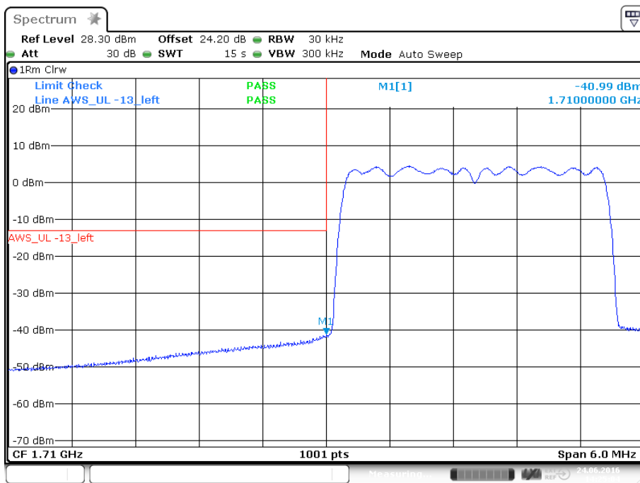
plot 7.3.4.1-#1 Intermodulation: §27.53, §2.1051; Test results; Uplink; CDMA Lower Band Edge
