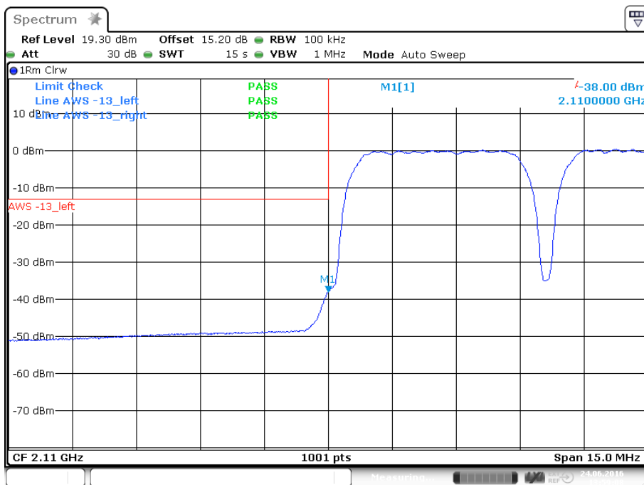
plot 7.3.3.2-#1 Intermodulation: §27.53, §2.1051; Test results; Downlink; WCDMA Lower Band Edge
