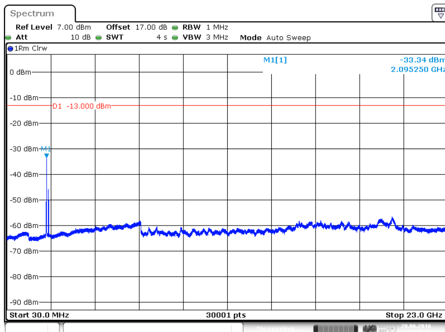
plot 6.3.3.2-#1 Spurious Emissions at Antenna Terminals: §27.53, §2.1051; Test results; Downlink; W-CDMA; carrier (2145MHz) notched
