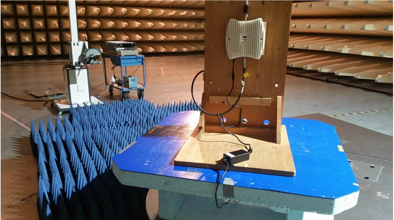
picture 8.4: Test setup: Field Strength Emission 18 – 26.5 GHz @3m in the SAC
