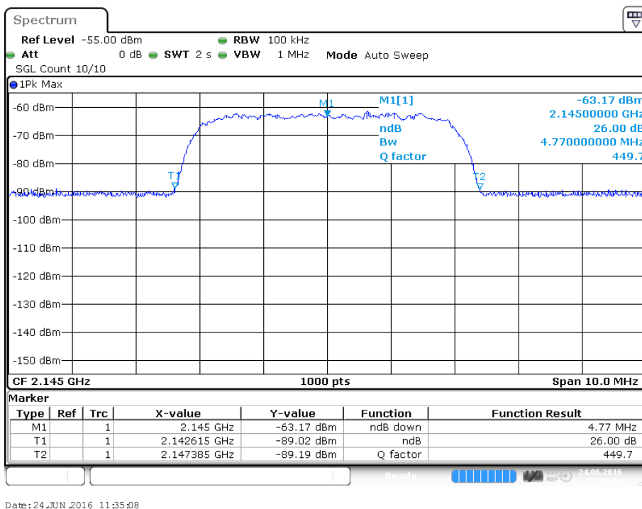
plot 5.3.4.2-#2 Occupied Bandwidth: §2.1049; Test results; 26dB Bandwidth; W-CDMA Input
