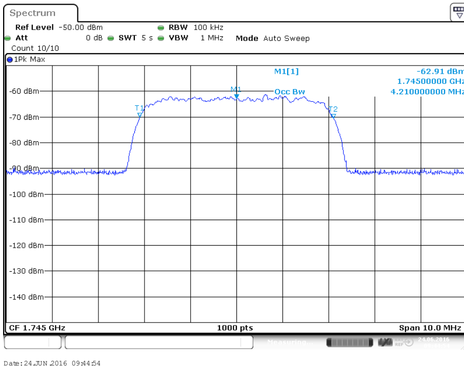
plot 5.3.5.2-#2 Occupied Bandwidth: 4.21000000 MHz; Test results; Uplink; W-CDMA Input
