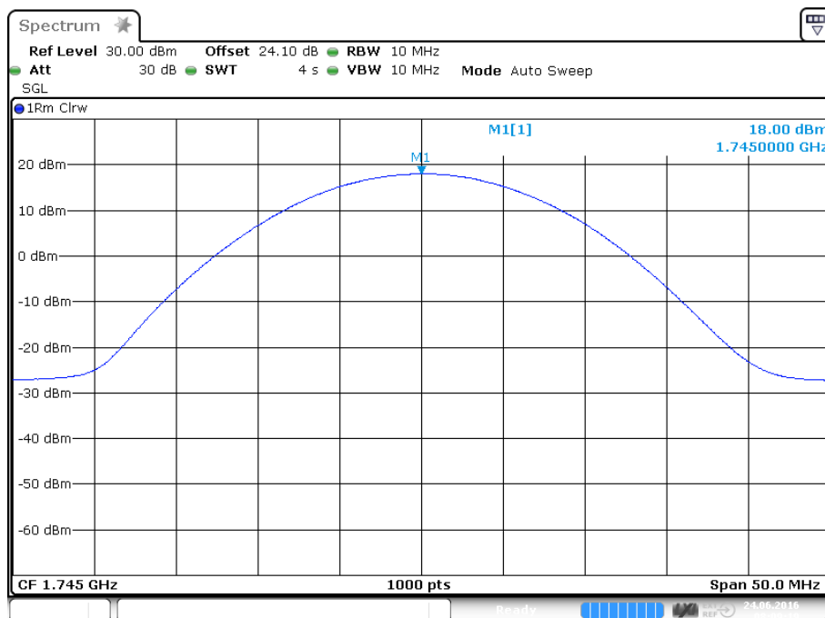
plot 4.3.4.2-#1 RF Power Out: §27.50, §2.1046; Test results; Uplink; W-CDMA Middle
