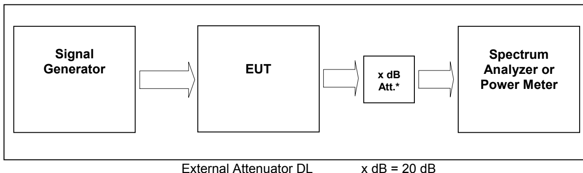
figure 4-#1 Test setup: RF Power Out: §27.50, §2.1046
