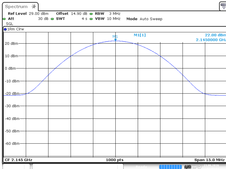
plot 4.3.3.1-#1 RF Power Out: §27.50, §2.1046; Test results; Downlink; CDMA Middle
