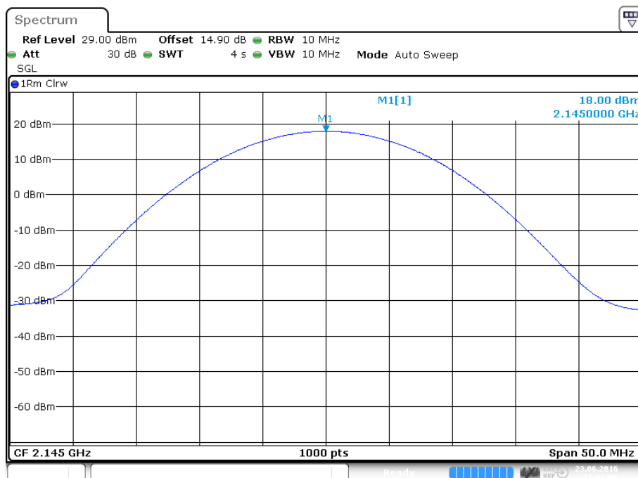
plot 4.3.3.2-#1 RF Power Out: §27.50, §2.1046; Test results; Downlink; W-CDMA Middle
