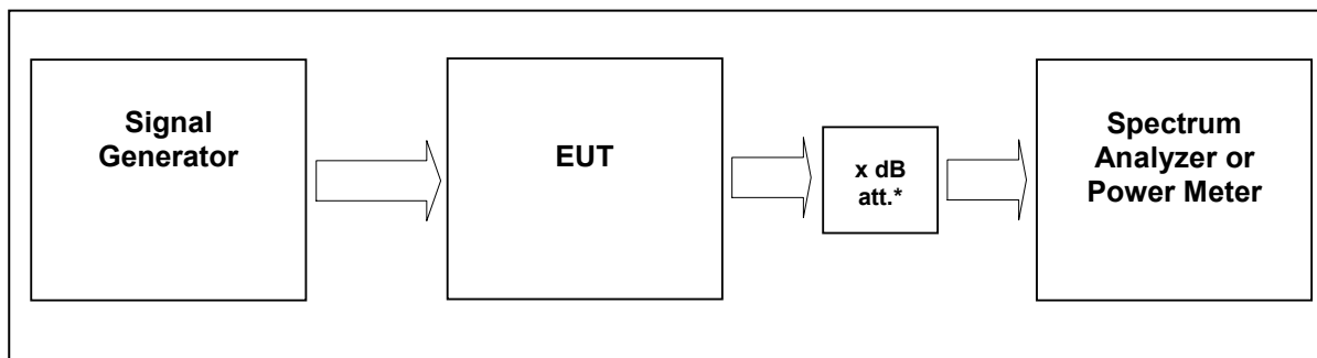
figure 6-#1 Test setup: Spurious Emissions at Antenna Terminals: §27.53, §2.1051
