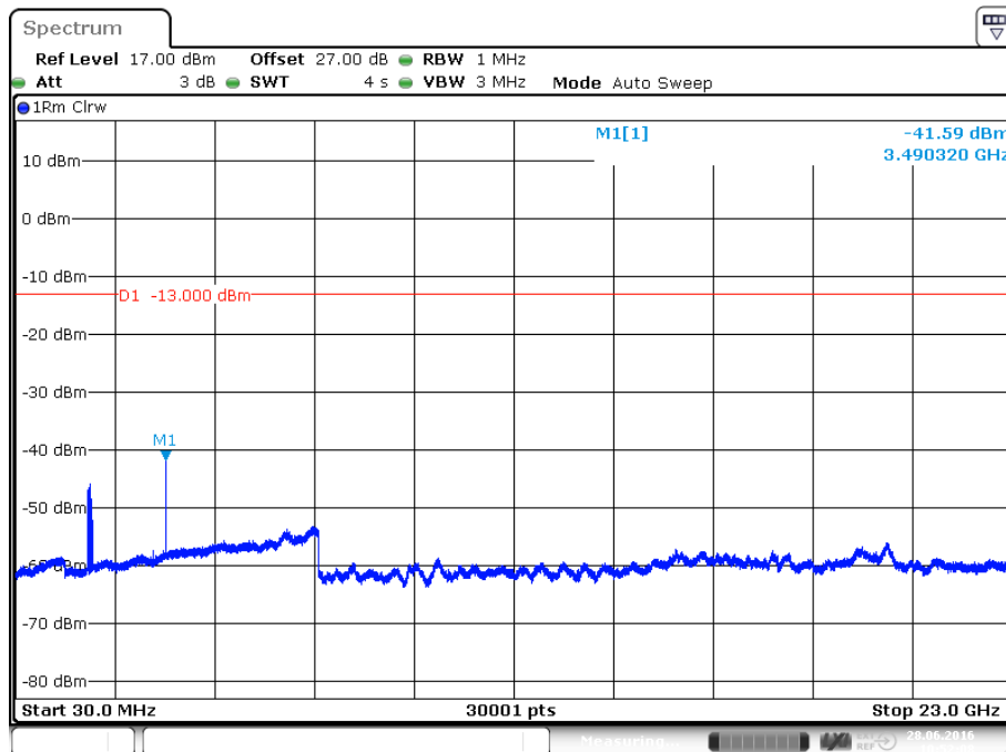
plot 6.3.4.1-#1 Spurious Emissions at Antenna Terminals: §27.53, §2.1051; Test results; Uplink; CDMA; carrier (2145MHz) notched
