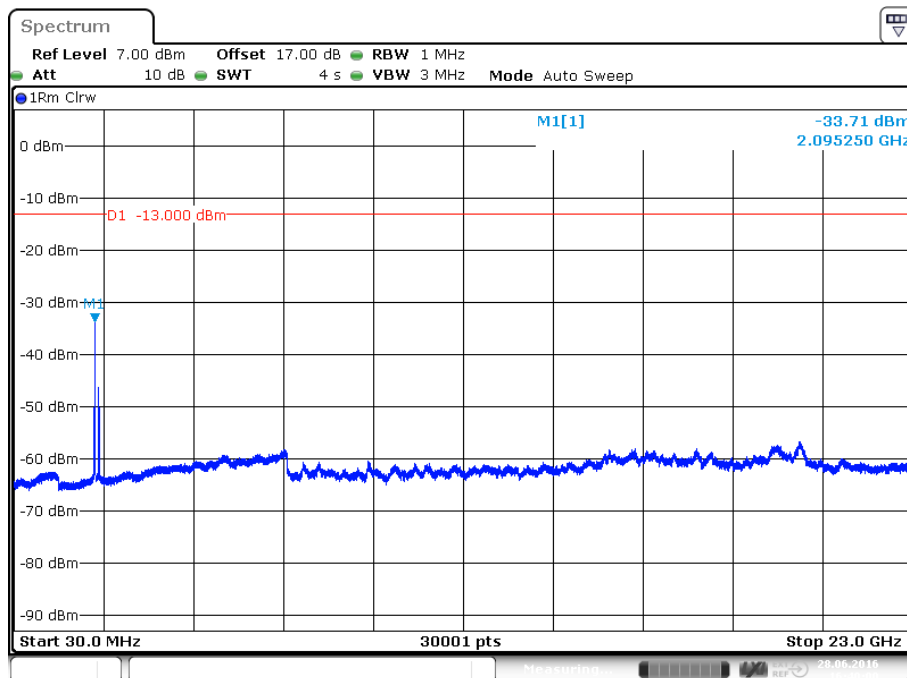
plot 6.3.3.1-#1 Spurious Emissions at Antenna Terminals: §27.53, §2.1051; Test results; Downlink; CDMA; carrier (2145MHz) notched
