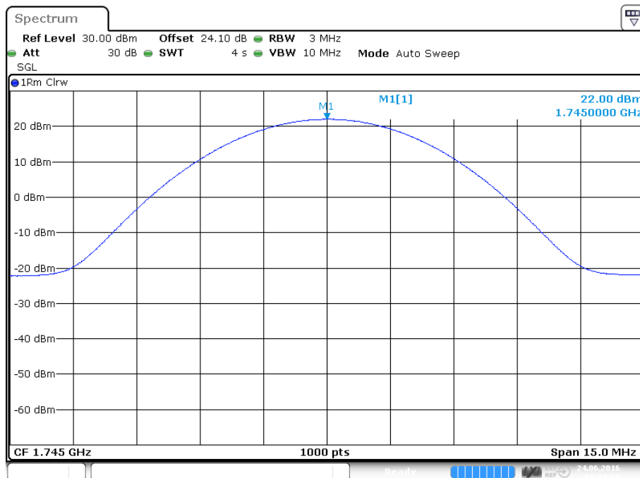
plot 4.3.4.1-#1 RF Power Out: §27.50, §2.1046; Test results; Uplink; CDMA Middle
