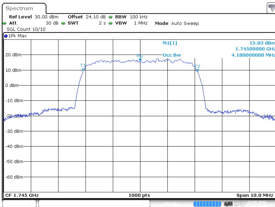
plot 5.3.5.2-#1 Occupied Bandwidth: 4.18000000 MHz; Test results; Uplink; W-CDMA Output
