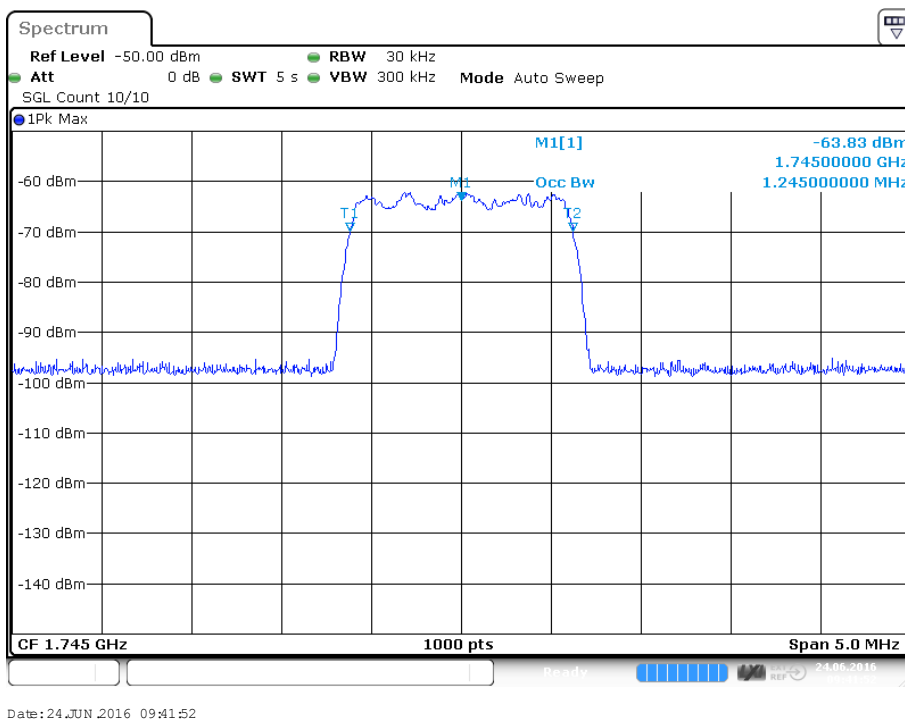
plot 5.3.5.1-#2 Occupied Bandwidth: §2.1049; Test results; Uplink; CDMA Input
