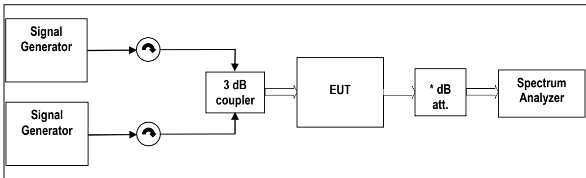
External Attenuator DL x dB = 20 dB figure 7-#1 Test setup: Intermodulation: §27.53, §2.1051
