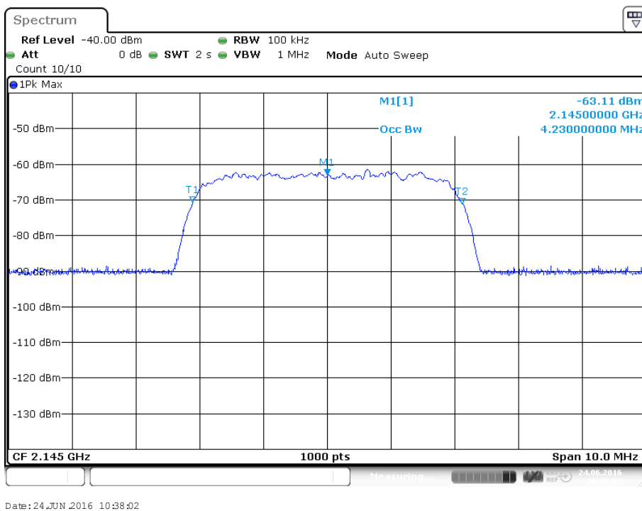
plot 5.3.3.2-#2 Occupied Bandwidth: §2.1049; Test results; Downlink; W-CDMA Input
