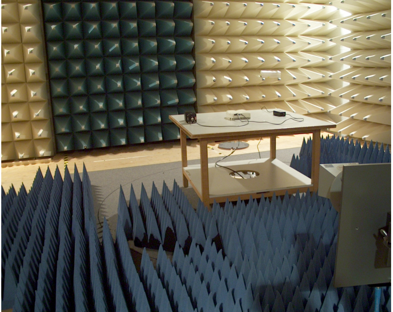
picture 8.3: Test setup: Field Strength Emission >20 GHz @3m in the FAC with Absorber material
