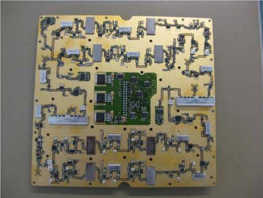
PCB Extension front
