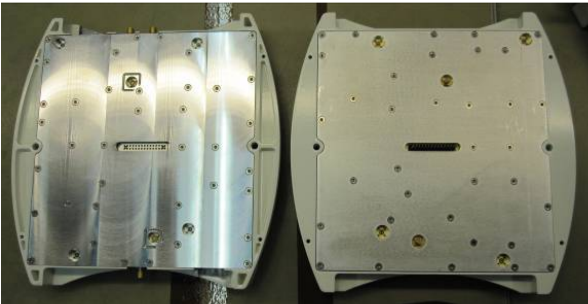
Main Unit back
