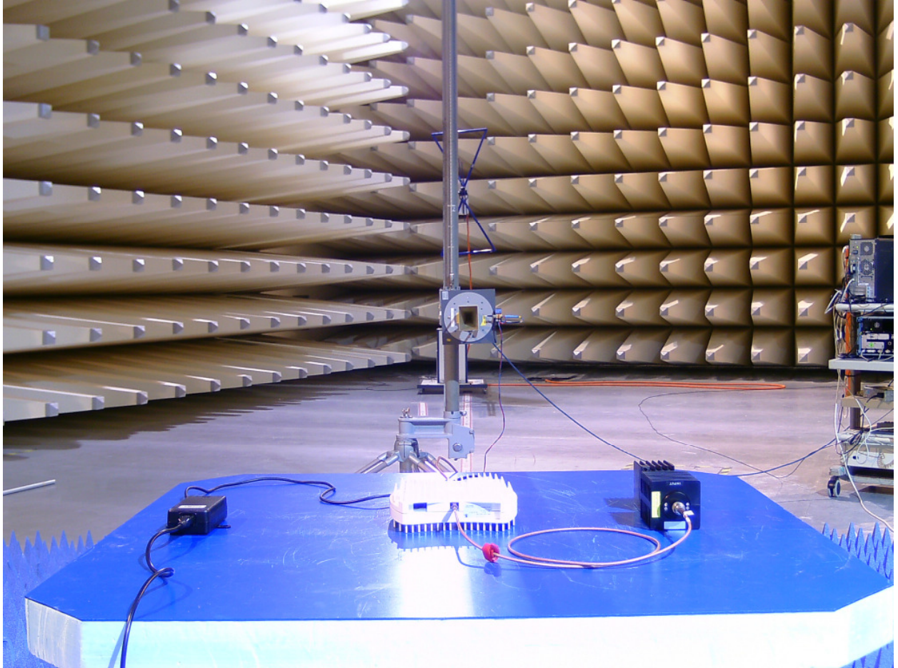
picture 8.3: Test setup: Field Strength Emission >20 GHz @3m in the SAC with Absorber material on the Groundplane
