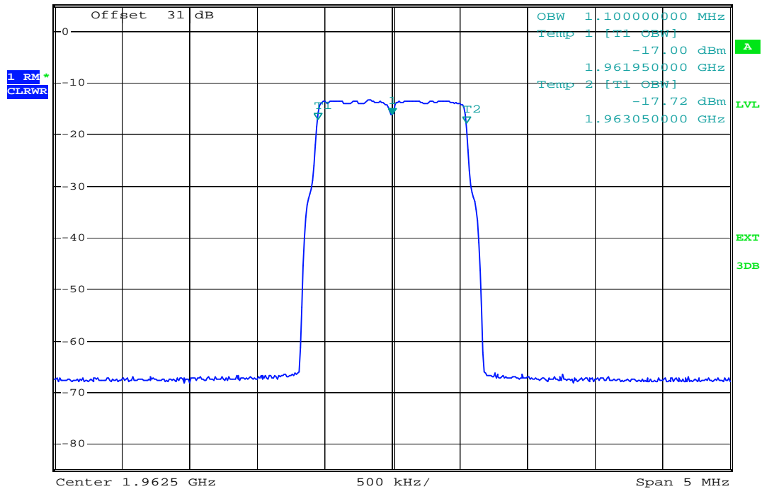
plot 6.3.1.5-#2 Occupied Bandwidth: §2.1049; RSS-GEN; Test results; Downlink; LTE Input
