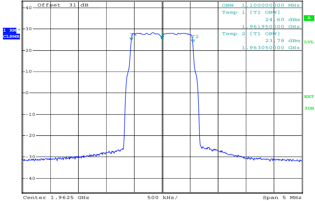
plot 6.3.1.5-#1 Occupied Bandwidth: §2.1049; RSS-GEN; Test results; Downlink; LTE Output
