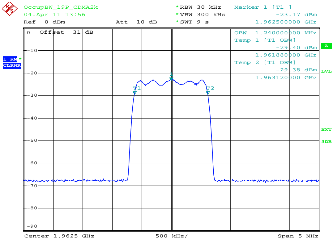
plot 6.3.1.1-#2 Occupied Bandwidth: §2.1049; RSS-GEN; Test results; Downlink; CDMA Input
