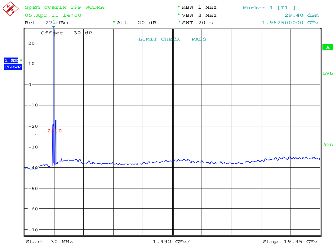
plot 7.3.1.7-#1 Spurious Emissions at Antenna Terminals: §24.238, §2.1051; RSS-132, RSS-GEN; Test results; Downlink; W-CDMA > 1MHz to band edge; carrier (1962,5MHz) notched
