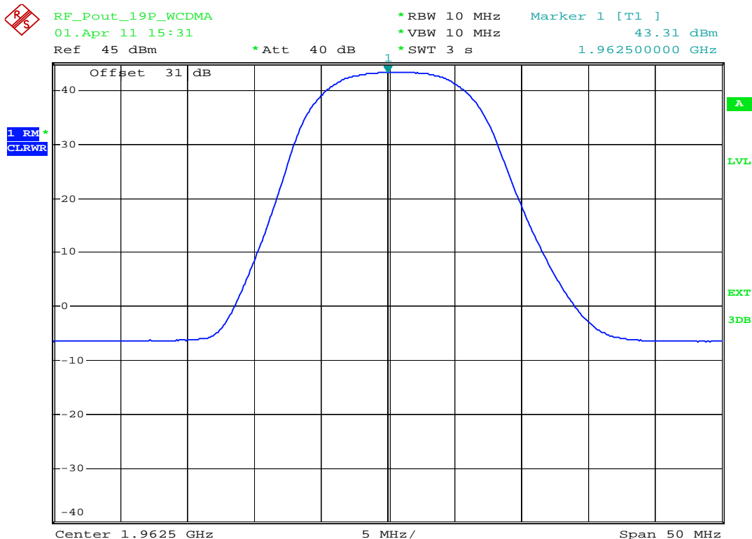
plot 5.3.1.4-#1 RF Power Out: §24.232, §2.1046; RSS-133, RSS-GEN; Test results; Downlink; W-CDMA Middle
