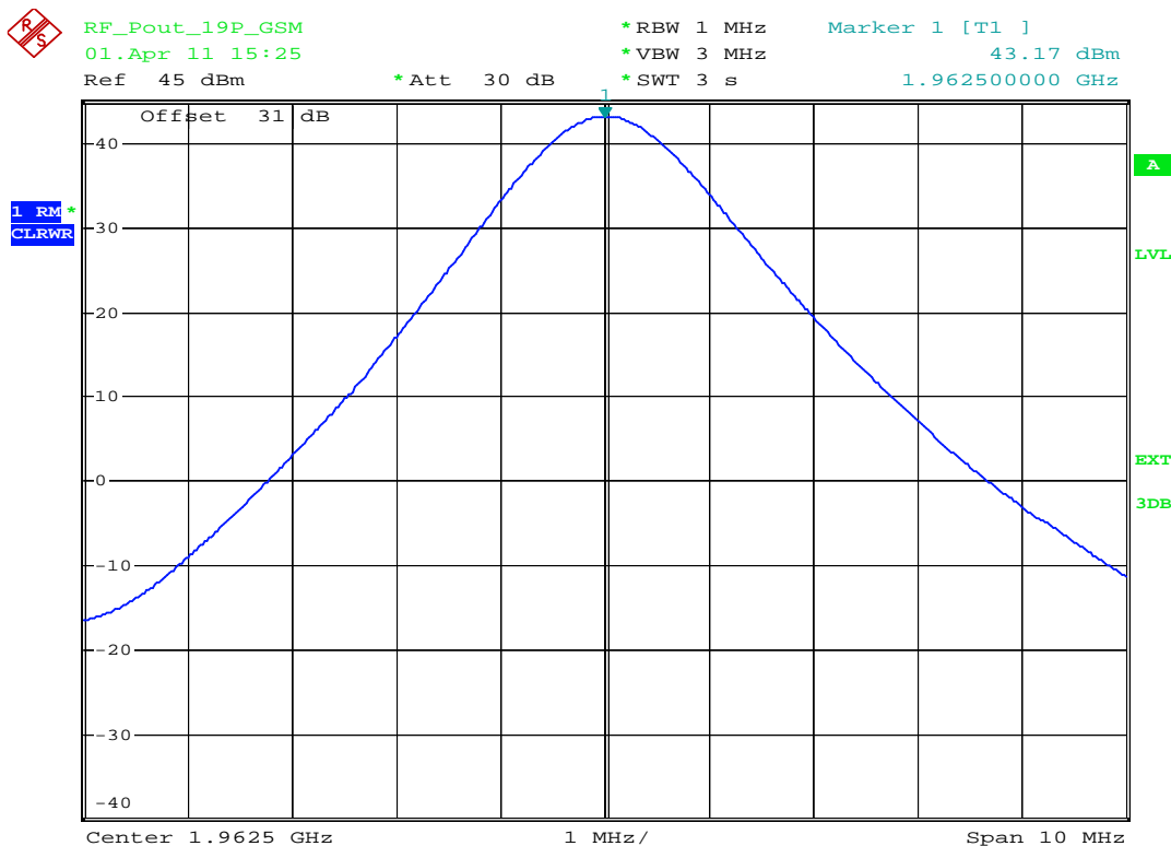
plot 5.3.1.1-#1 RF Power Out: §24.232, §2.1046; RSS-133, RSS-GEN; Test results; Downlink; GSM Middle
