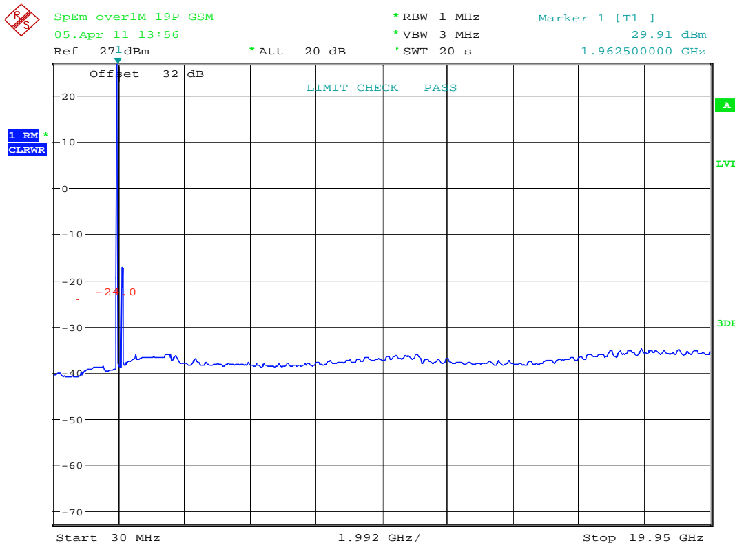
plot 7.3.1.8-#1 Spurious Emissions at Antenna Terminals: §24.238, §2.1051; RSS-132, RSS-GEN; Test results; Downlink; GSM > 1MHz to band edge; carrier (1962,5MHz) notched
