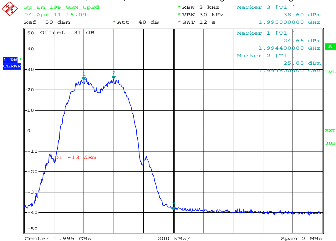
plot 7.3.1.3-#2 Spurious Emissions at Antenna Terminals: §24.238, §2.1051; RSS-132, RSS-GEN; Test results; Downlink; GSM < 1MHz to band edge Upper Band Edge
