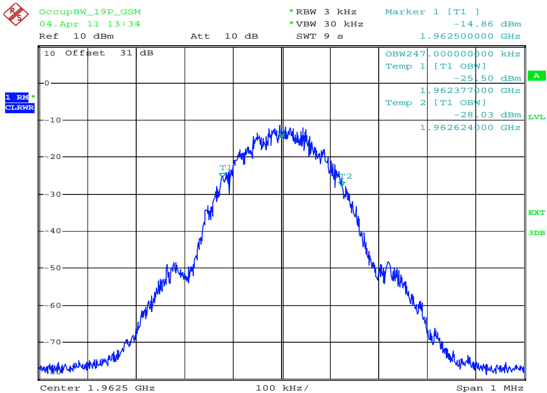
plot 6.3.1.3-#2 Occupied Bandwidth: §2.1049; RSS-GEN; Test results; Downlink; GSM Input
