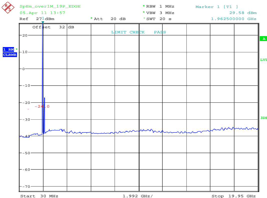
plot 7.3.1.9-#1 Spurious Emissions at Antenna Terminals: §24.238, §2.1051; RSS-132, RSS-GEN; Test results; Downlink; GSM-EDGE > 1MHz to band edge; carrier (1962,5MHz) notched
