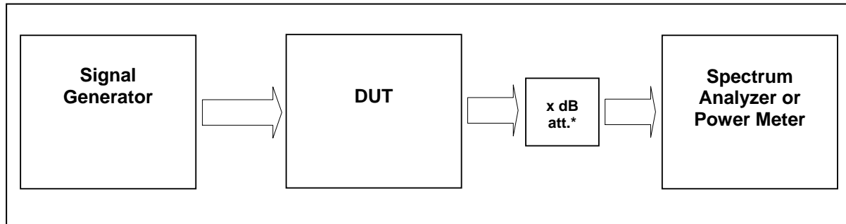
External Attenuator DL x dB = 10 dB figure 5.4-#1 Test setup: Occupied Bandwidth: §2.1049; RSS-GEN
