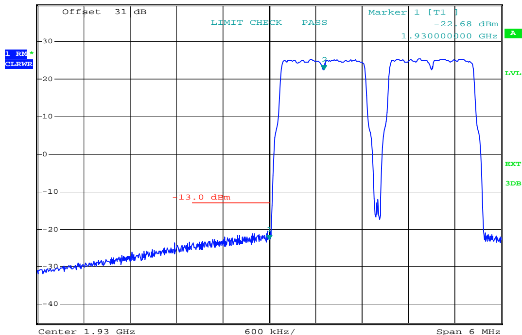
plot 7.3.1.5-#1 Spurious Emissions at Antenna Terminals: §24.238, §2.1051; RSS-132, RSS-GEN; Test results; Downlink; LTE < 1MHz to band edge Lower Band Edge
