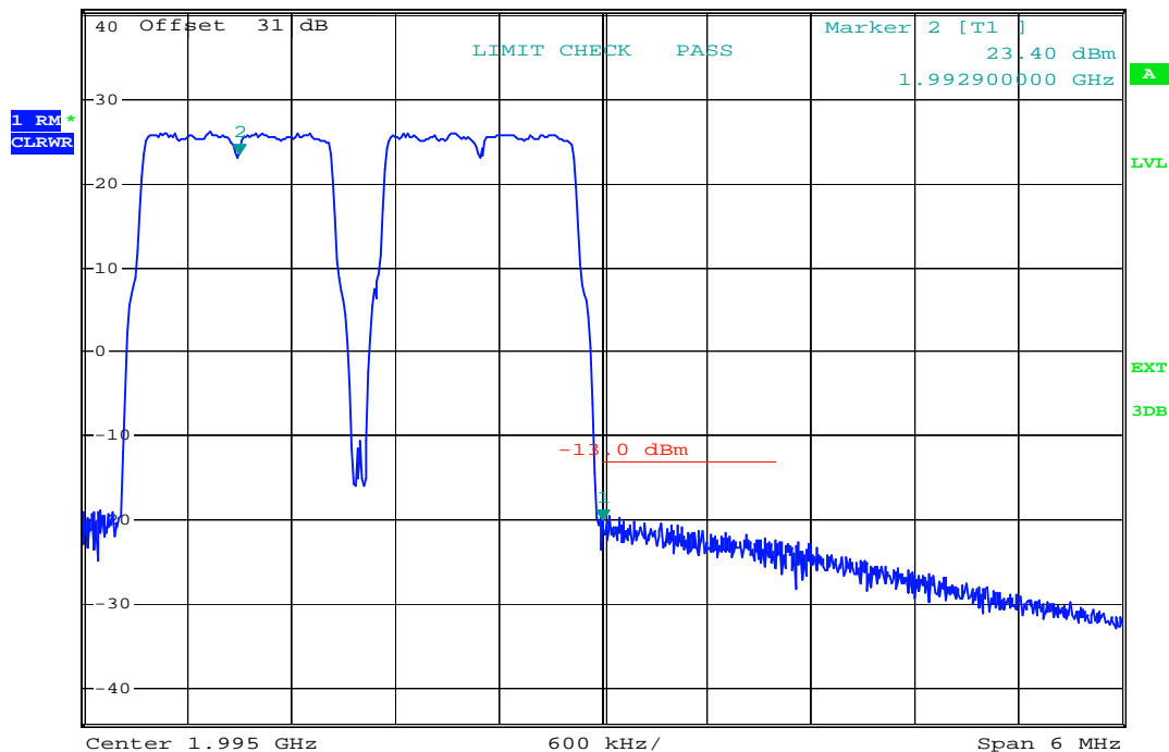
plot 7.3.1.5-#2 Spurious Emissions at Antenna Terminals: §24.238, §2.1051; RSS-132, RSS-GEN; Test results; Downlink; LTE < 1MHz to band edge Upper Band Edge
