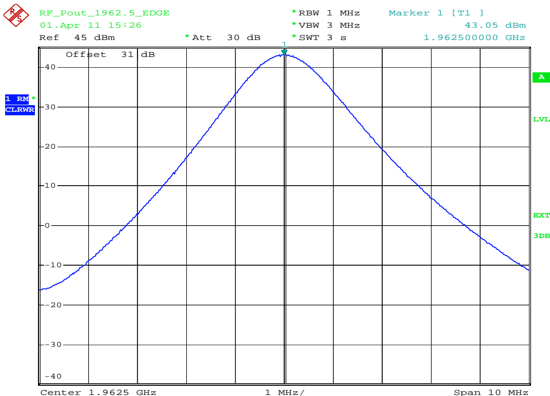
plot 5.3.1.2-#1 RF Power Out: §24.232, §2.1046; RSS-133, RSS-GEN; Test results; Downlink; GSM-EDGE Middle
