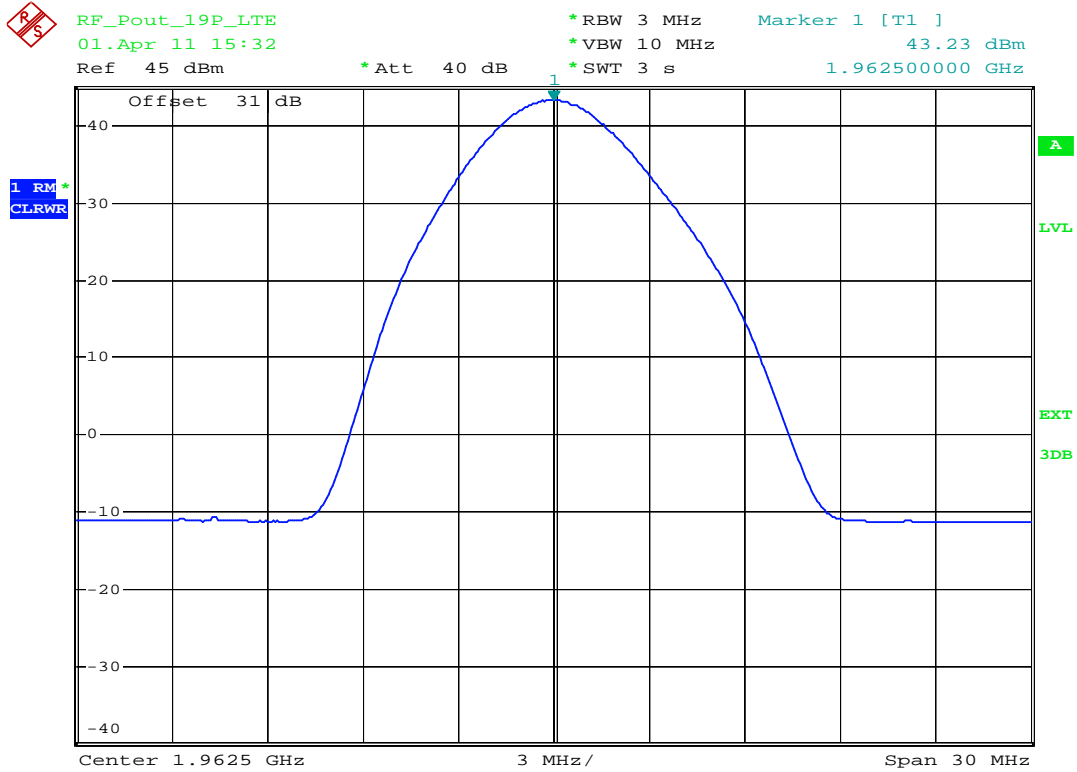
plot 5.3.1.5-#1 RF Power Out: §24.232, §2.1046; RSS-133, RSS-GEN; Test results; Downlink; LTE Middle
