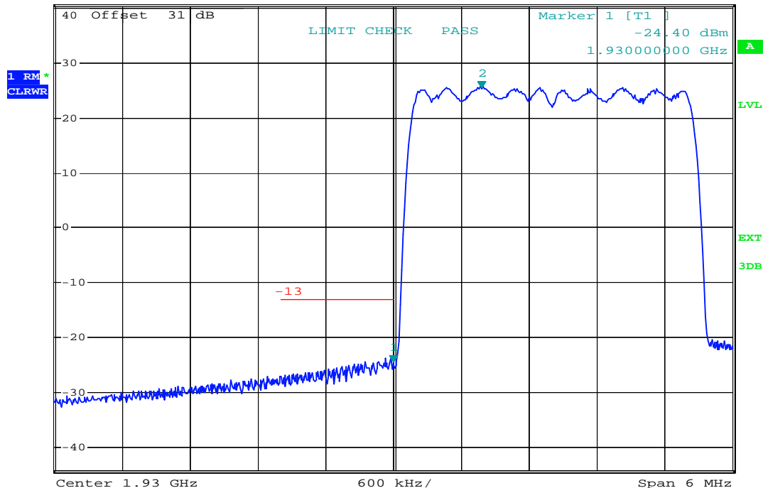
plot 7.3.1.1-#1 Spurious Emissions at Antenna Terminals: §24.238, §2.1051; RSS-132, RSS-GEN; Test results; Downlink; CDMA < 1MHz to band edge Lower Band Edge
