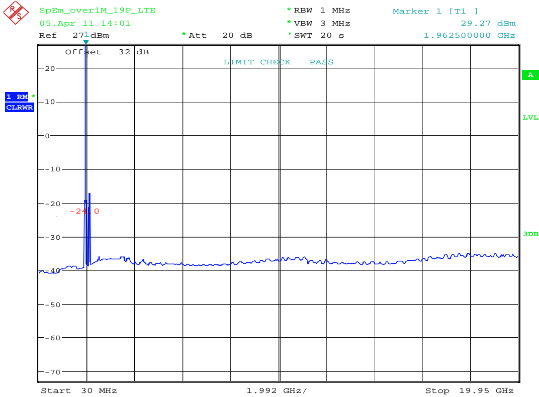
plot 7.3.1.10-#1 Spurious Emissions at Antenna Terminals: §24.238, §2.1051; RSS-132, RSS-GEN; Test results; Downlink; LTE > 1MHz to band edge; carrier (1962,5MHz) notched
