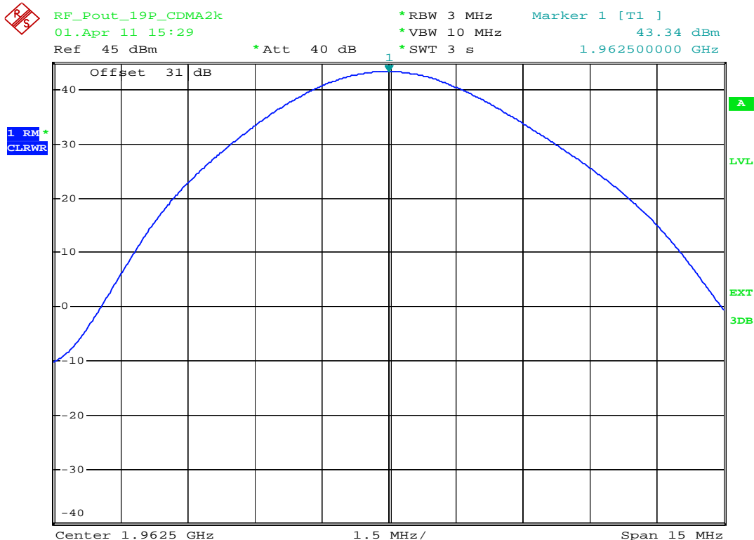
plot 5.3.1.3-#1 RF Power Out: §24.232, §2.1046; RSS-133, RSS-GEN; Test results; Downlink; CDMA Middle
