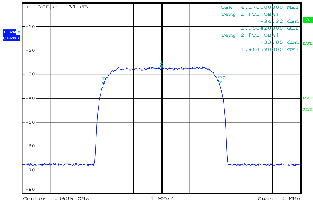
plot 6.3.1.2-#2 Occupied Bandwidth: §2.1049; RSS-GEN; Test results; Downlink; W-CDMA Input
