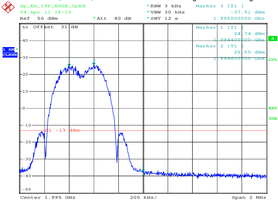
plot 7.3.1.4-#2 Spurious Emissions at Antenna Terminals: §24.238, §2.1051; RSS-132, RSS-GEN; Test results; Downlink; GSM-EDGE < 1MHz to band edge Upper Band Edge
