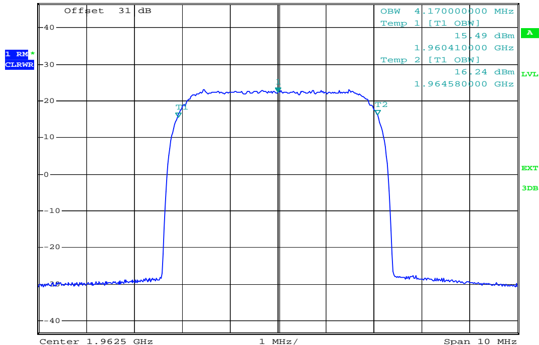
plot 6.3.1.2-#1 Occupied Bandwidth: §2.1049; RSS-GEN; Test results; Downlink; W-CDMA Output
