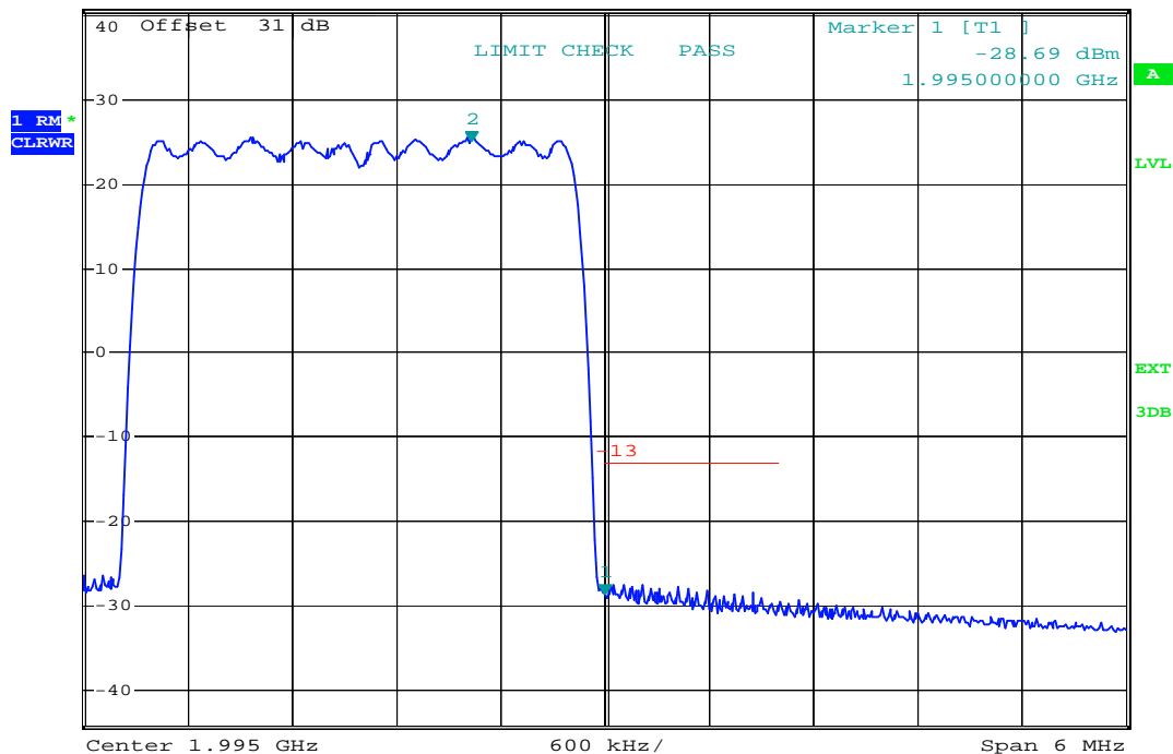
plot 7.3.1.1-#2 Spurious Emissions at Antenna Terminals: §24.238, §2.1051; RSS-132, RSS-GEN; Test results; Downlink; CDMA < 1MHz to band edge Upper Band Edge
