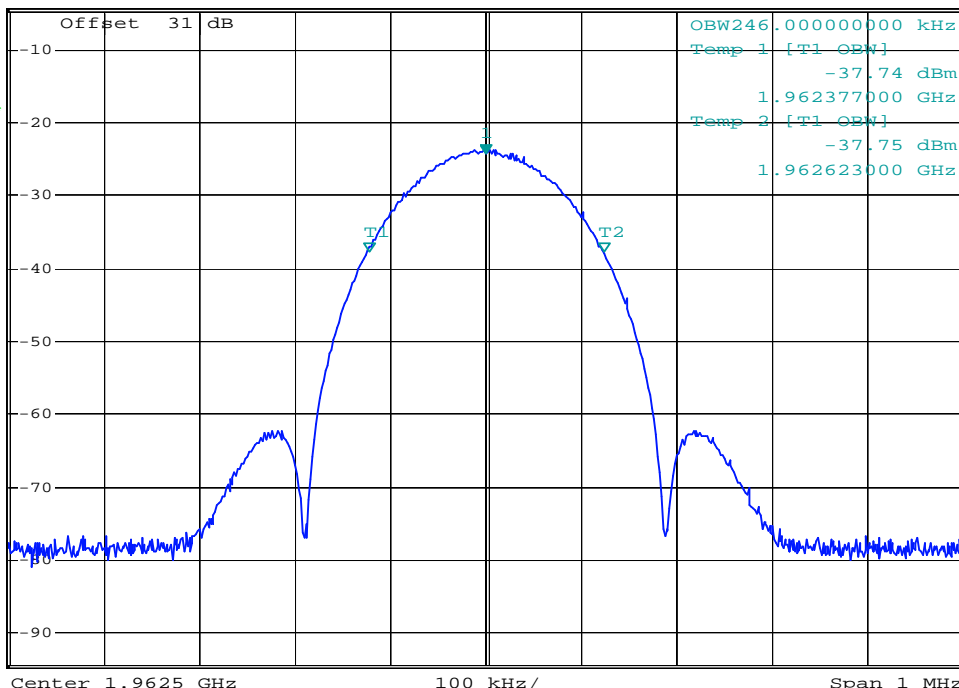
plot 6.3.1.4-#2 Occupied Bandwidth: §2.1049; RSS-GEN; Test results; Downlink; GSM-EDGE Input
