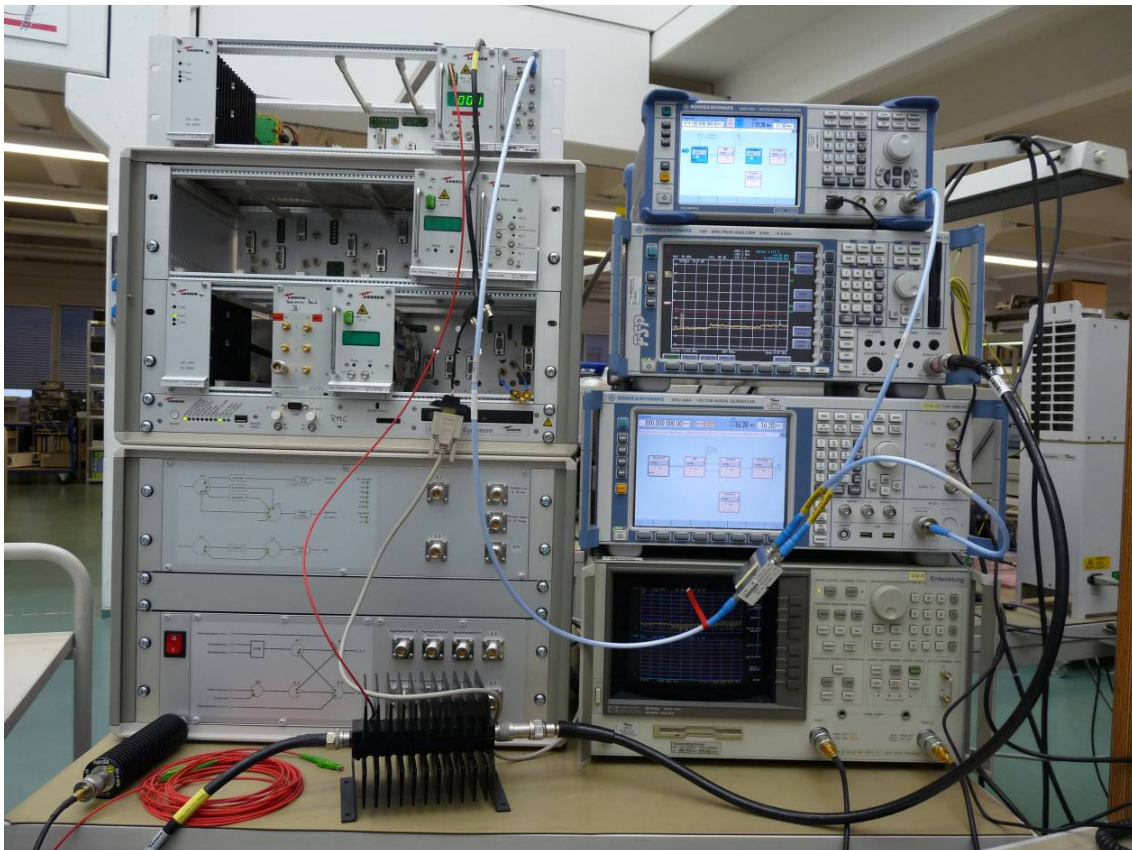
Figure 2. Measurement Equipment
