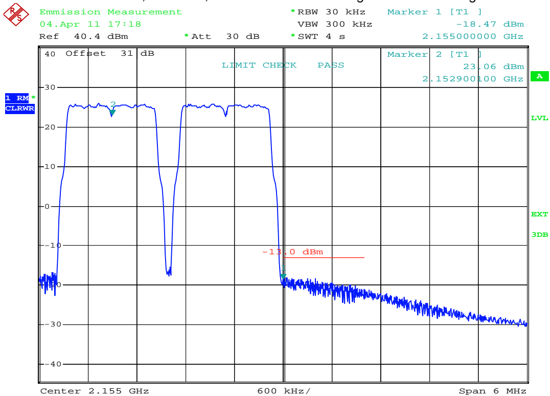
plot 7.3.1.3-#2 Spurious Emissions at Antenna Terminals: §27.53, §2.1051; RSS-139, RSS-GEN; Test results; Downlink; LTE < 1MHz to band edge Upper Band Edge
