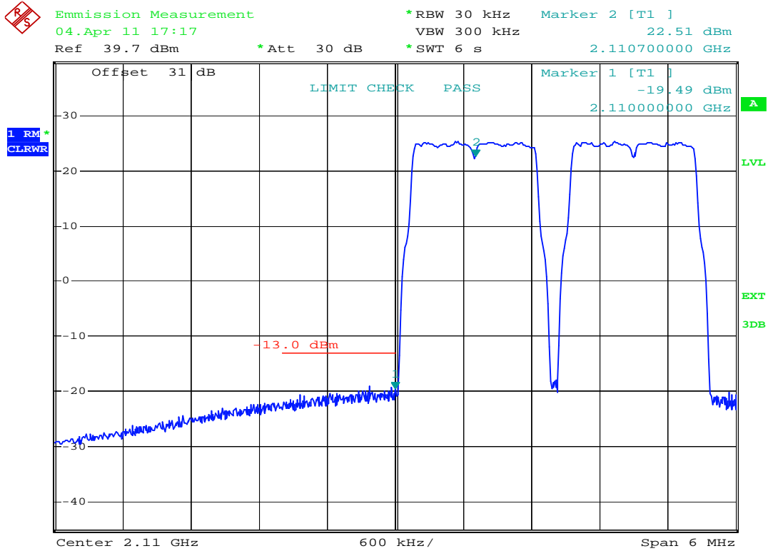
plot 7.3.1.3-#1 Spurious Emissions at Antenna Terminals: §27.53, §2.1051; RSS-139, RSS-GEN; Test results; Downlink; LTE < 1MHz to band edge Lower Band Edge
