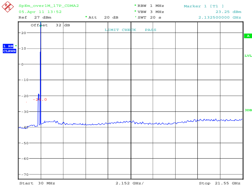
plot 7.3.1.4-#1 Spurious Emissions at Antenna Terminals: §27.53, §2.1051; RSS-139, RSS-GEN; Test results; Downlink; CDMA > 1MHz to band edge; carrier (2132,5MHz) notched
