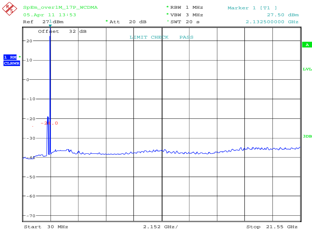
plot 7.3.1.5-#1 Spurious Emissions at Antenna Terminals: §27.53, §2.1051; RSS-139, RSS-GEN; Test results; Downlink; W-CDMA > 1MHz to band edge; carrier (2132,5MHz) notched
