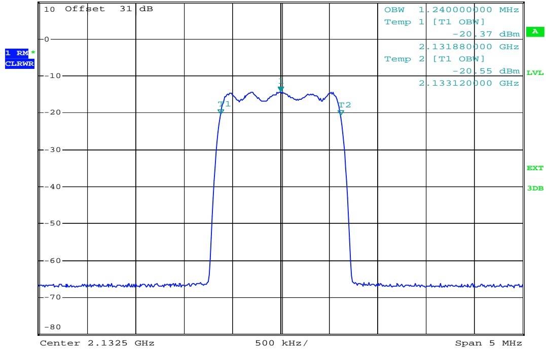
plot 6.3.1.1-#2 Occupied Bandwidth: §2.1049; RSS-GEN; Test results; Downlink; CDMA Input
