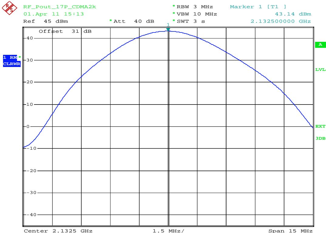
plot 5.3.1.1-#1 RF Power Out: §27.50, §2.1046; RSS-139, RSS-GEN; Test results; Downlink; CDMA Middle
