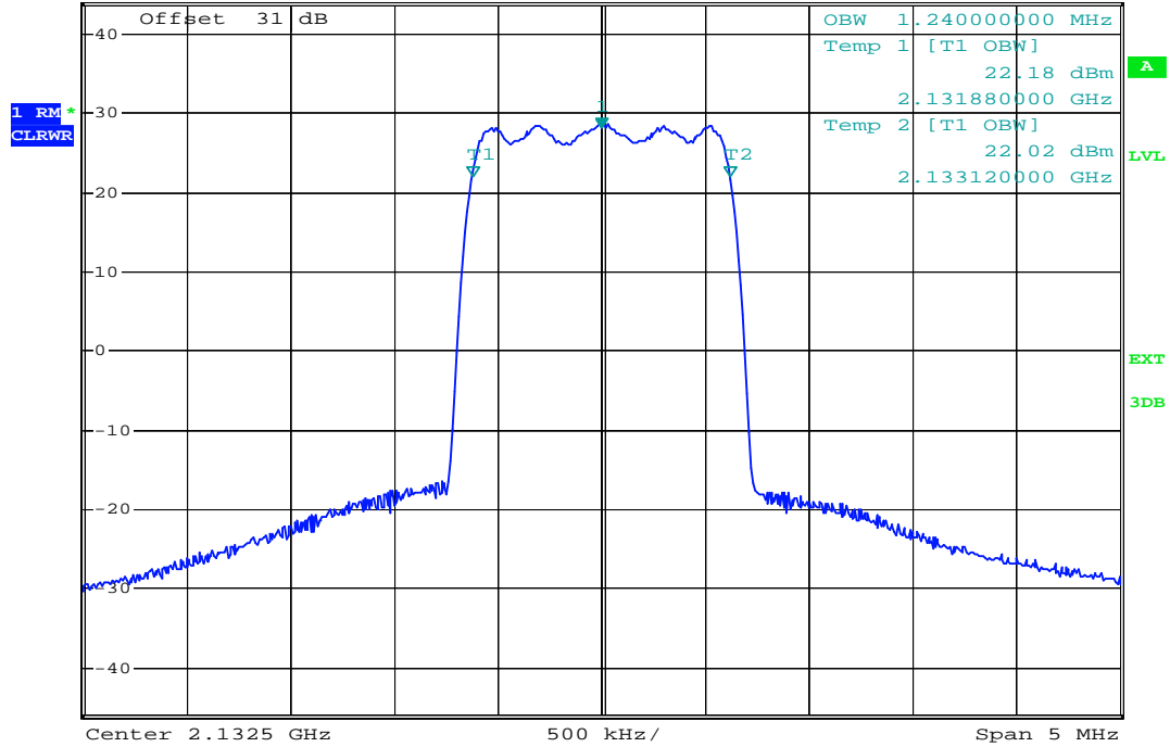
plot 6.3.1.1-#1 Occupied Bandwidth: §2.1049; RSS-GEN; Test results; Downlink; CDMA Output
