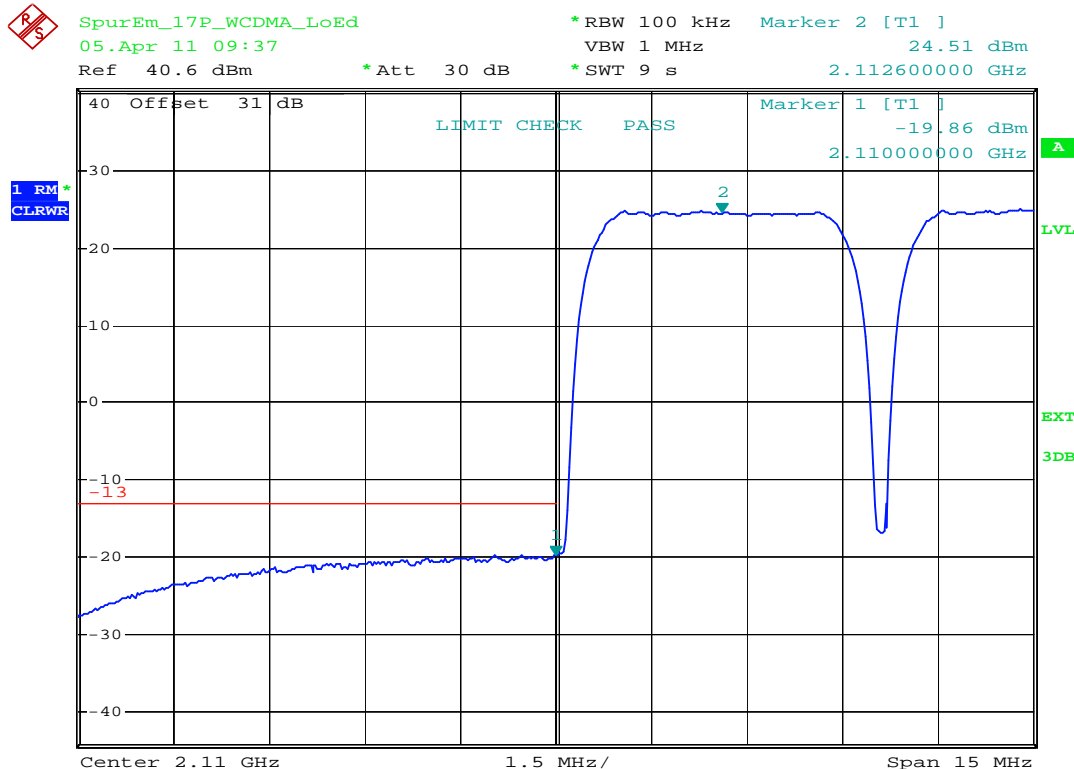
plot 7.3.1.1-#1 Spurious Emissions at Antenna Terminals: §27.53, §2.1051; RSS-139, RSS-GEN; Test results; Downlink; WCDMA < 1MHz to band edge Lower Band Edge
