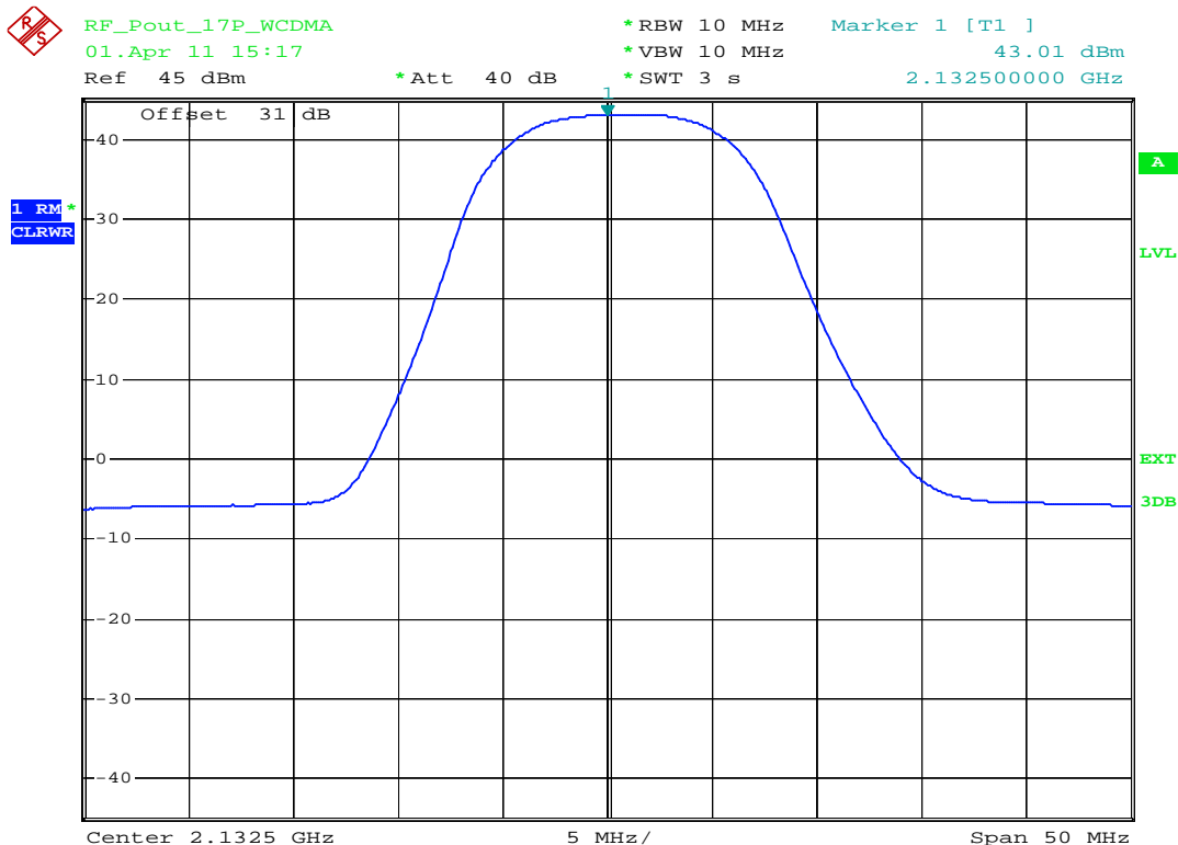
plot 5.3.1.2-#1 RF Power Out: §27.50, §2.1046; RSS-139, RSS-GEN; Test results; Downlink; W-CDMA Middle
