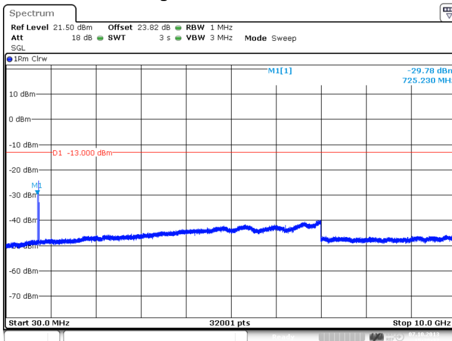
plot 7.3.1.4-#1 Spurious Emissions at Antenna Terminals: §27.53, §2.1051; Test results; Downlink; LTE > 1MHz to band edge 746 – 757MHz; 30 MHz – 10 GHz
