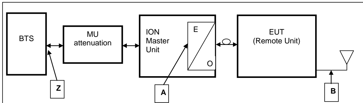
figure 2.1.4-#2 Block diagram of measurement reference points
