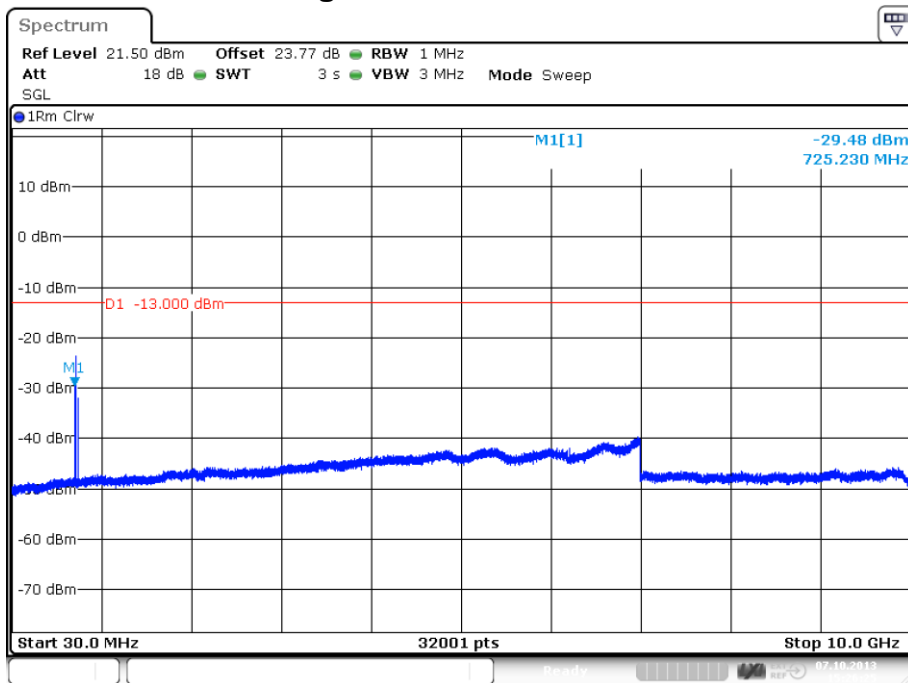
plot 7.3.1.3-#1 Spurious Emissions at Antenna Terminals: §27.53, §2.1051; Test results; Downlink; LTE > 1MHz to band edge 728 – 746MHz; 30 MHz – 10 GHz
