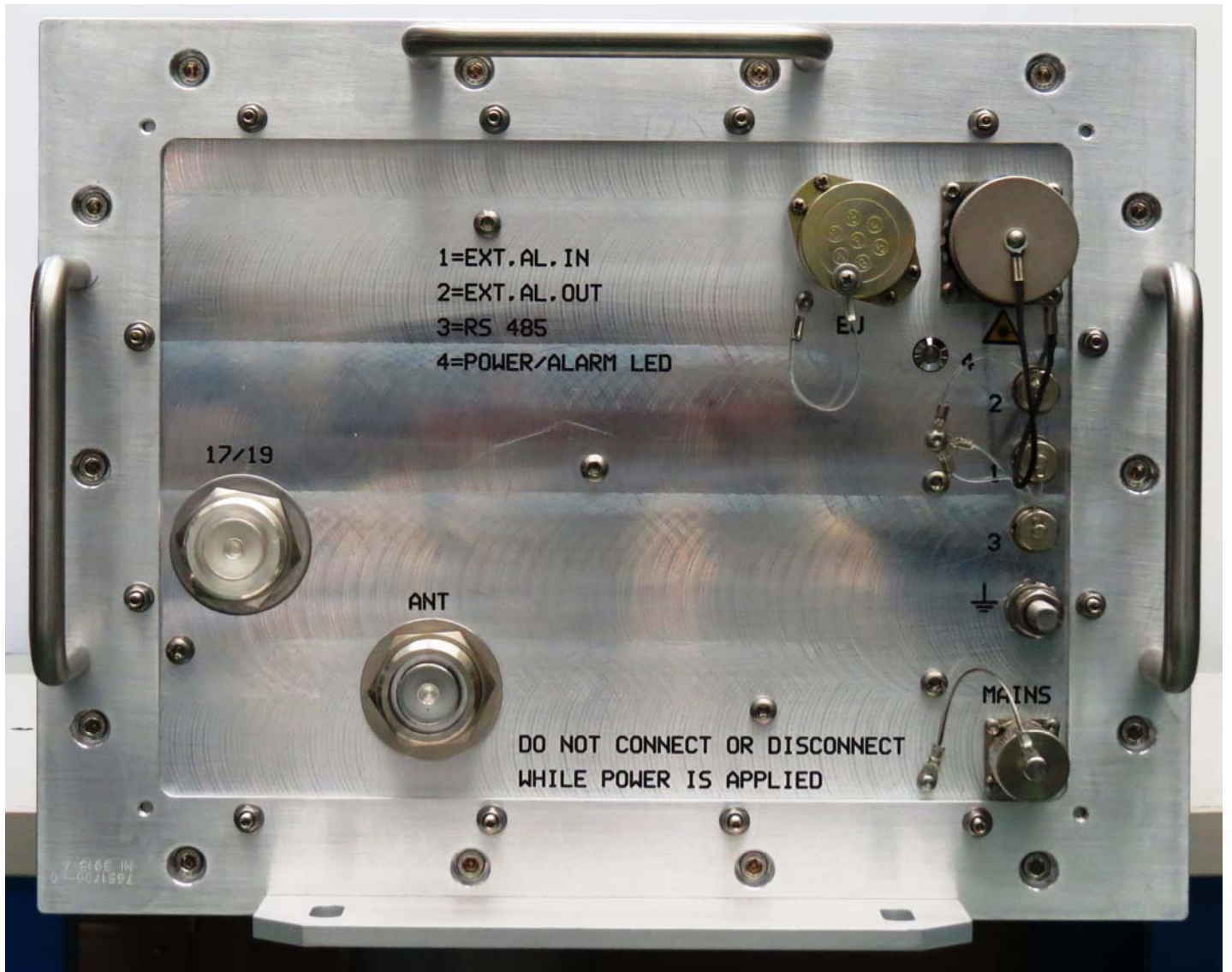
Connector flange (down side)
