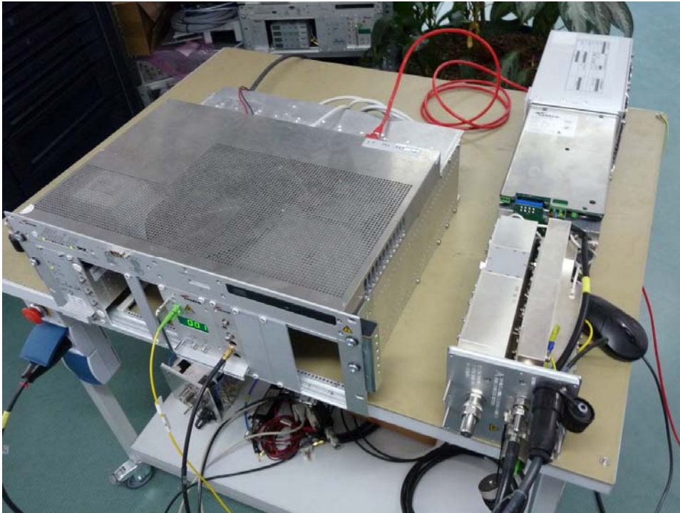
Figure 1. EUT ION-M7P/17HP
