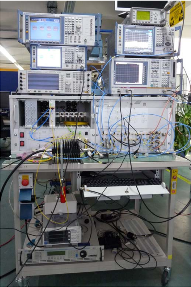
Figure 2. Measurement Equipment
