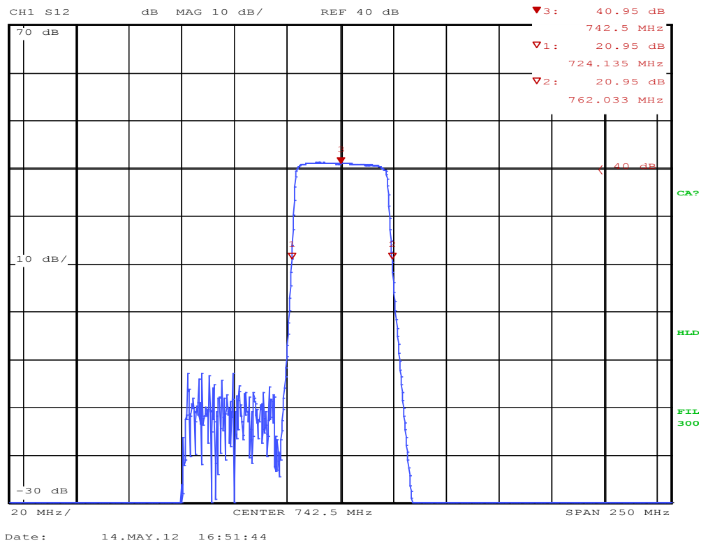
plot 8.3.1-#1 Amplifier Gain and Bandwidth: IC RSS-131; Test results; Downlink
