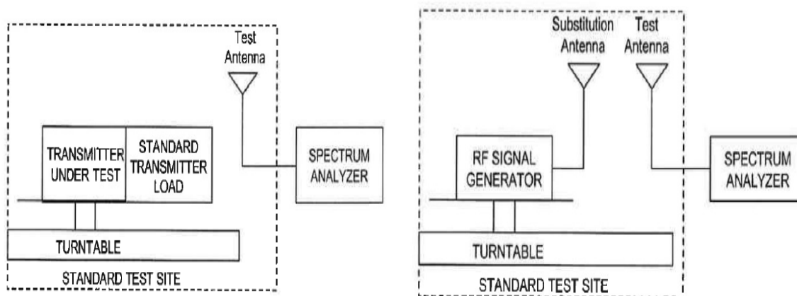
Figure #8.3 Substitution methods TIA/EIA-603-C
