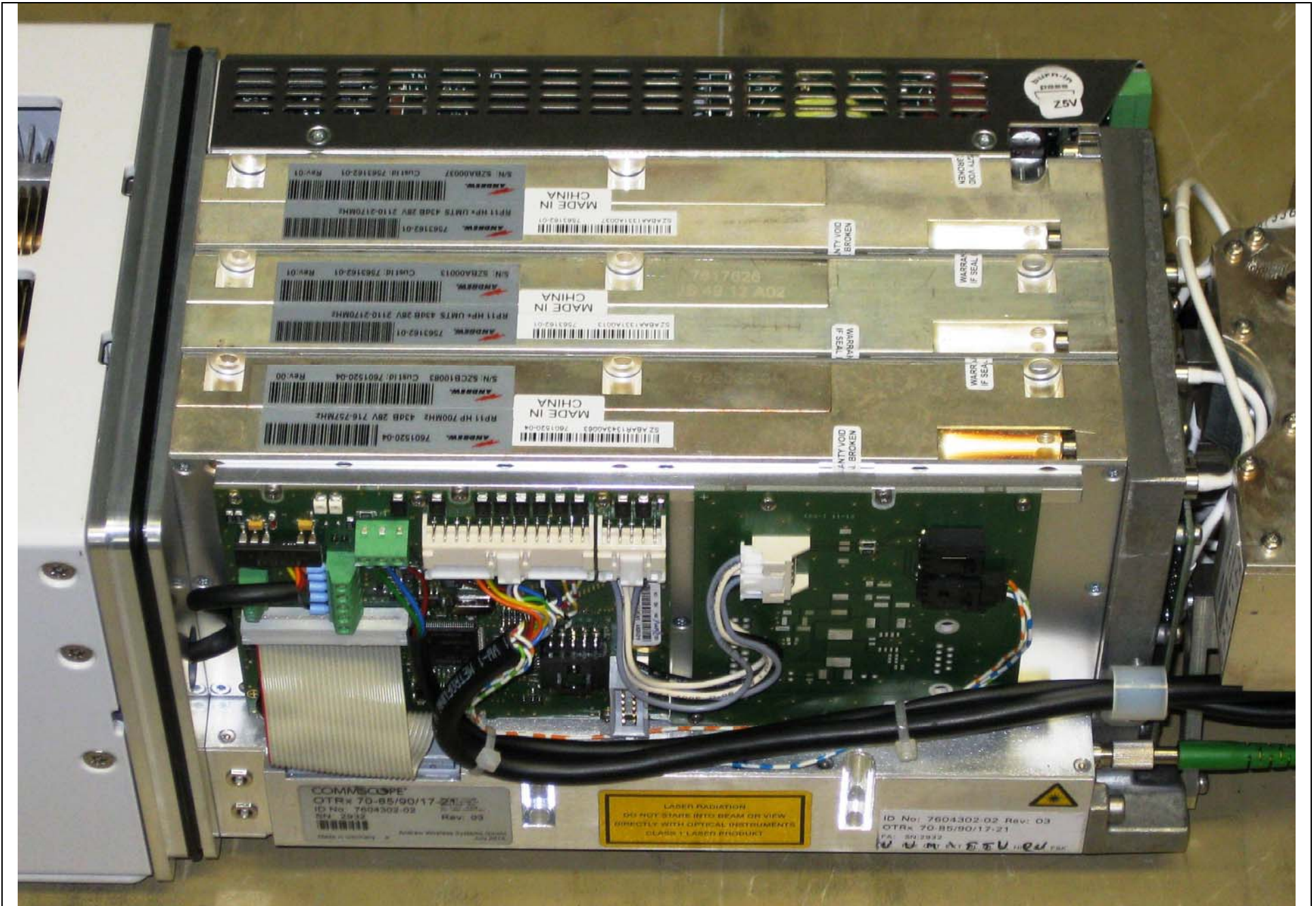
Amplifier
