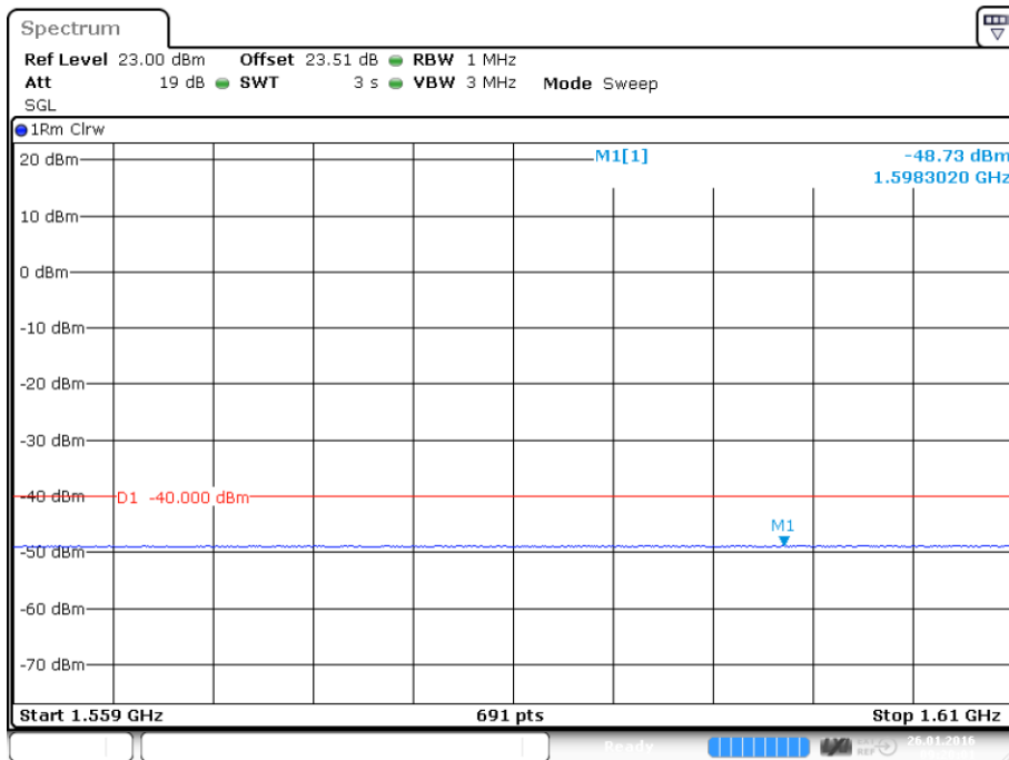
plot 7.3.1.3-#1 Spurious Emissions at Antenna Terminals: §27.53, §2.1051; Test results; Downlink; Measurement in the band of 1559 MHz – 1610 MHz acc. to 27.53(f); LTE band 12
