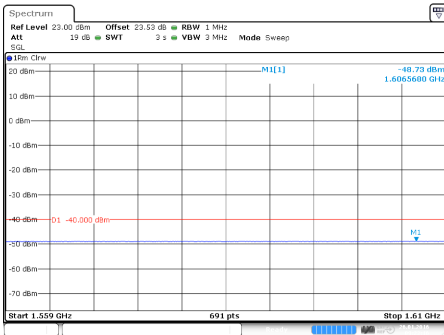
plot 7.3.1.3-#2 Spurious Emissions at Antenna Terminals: §27.53, §2.1051; Test results; Downlink; Measurement in the band of 1559 MHz – 1610 MHz acc. to 27.53(f); LTE band 13
