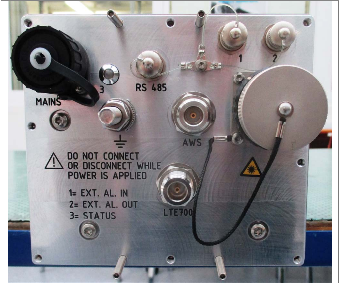
Front Flange
