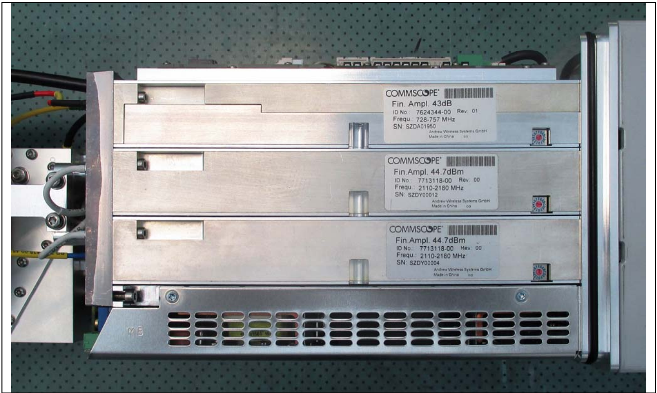
Amplifier
