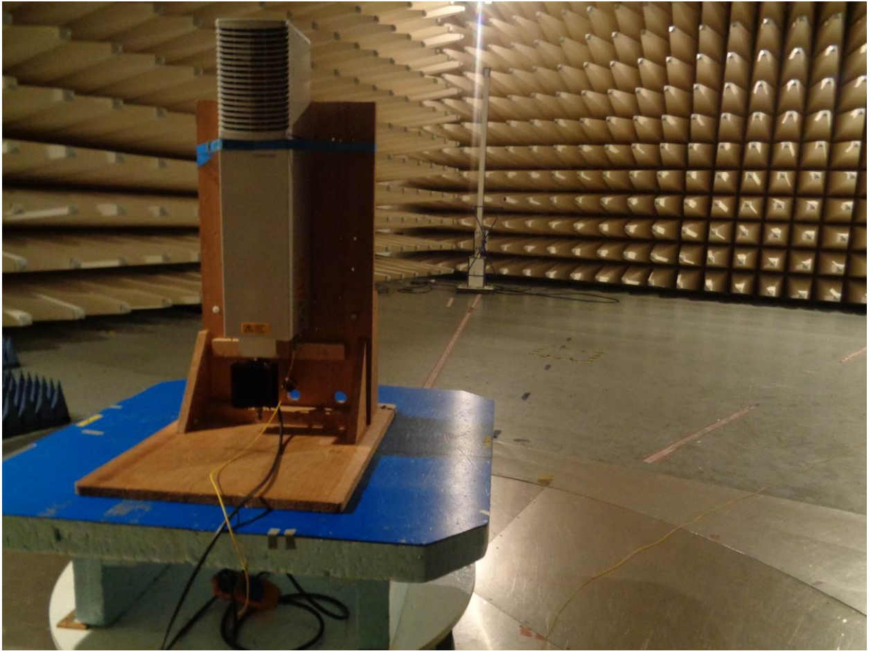
Test setup: Field Strength Emission 30 M – 1 GHz @10m in the SAC
