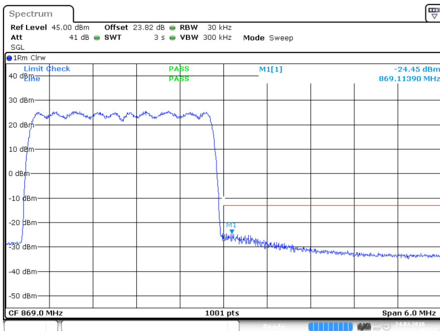
plot 8.3.1.3-#2 Intermodulation: §90.219, §2.1051; Test results; Downlink; CDMA Upper Band Edge
