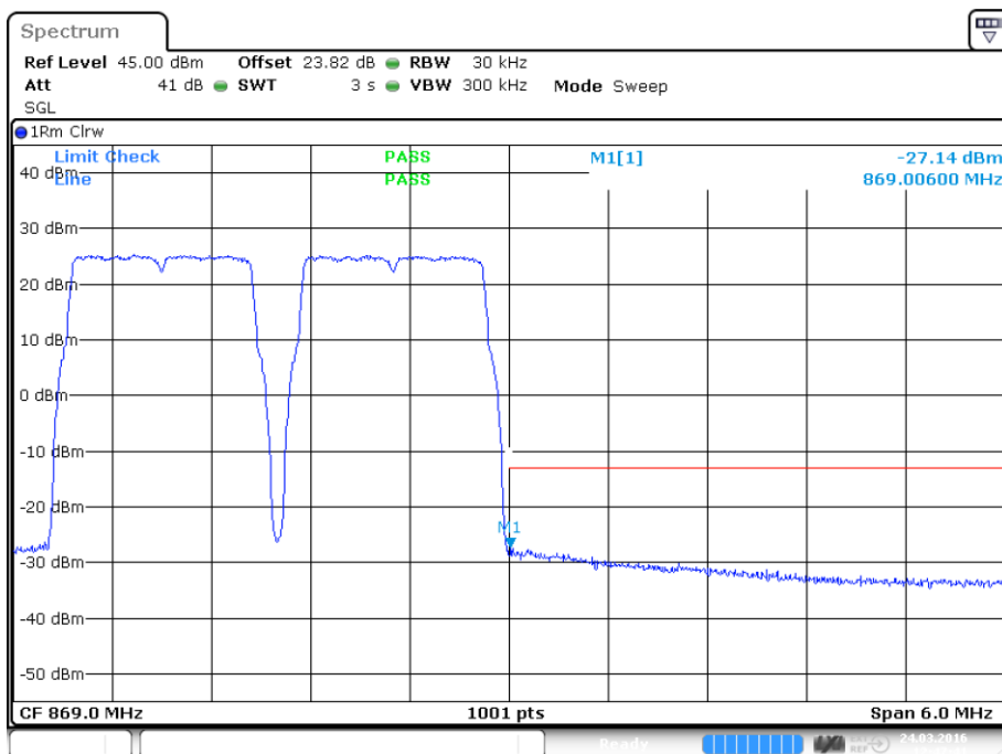
plot 8.3.1.5-#2 Intermodulation: §90.219, §2.1051; Test results; Downlink; LTE Upper Band Edge
