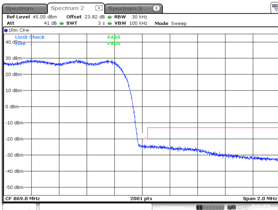
plot 9.3.1.3-#2 Emission Mask: §90.691, §2.1051; Test results; Downlink; CDMA Upper Band Edge
