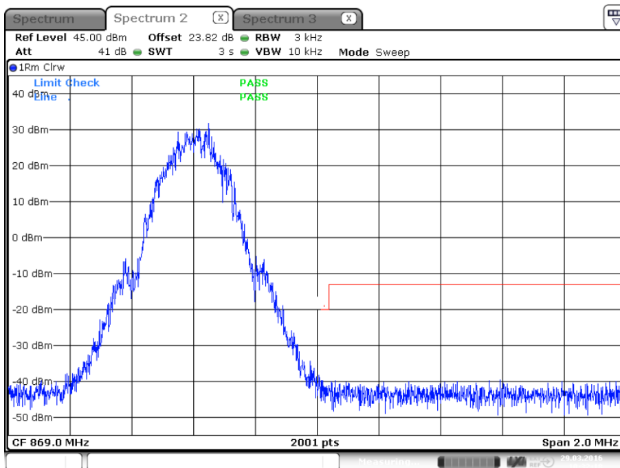
plot 9.3.1.1-#2 Emission Mask: §90.691, §2.1051; Test results; Downlink; GSM Upper Band Edge
