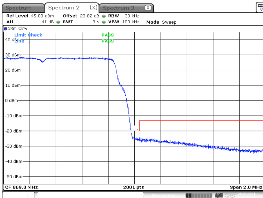
plot 9.3.1.5-#2 Emission Mask: §90.691, §2.1051; Test results; Downlink; LTE Upper Band Edge
