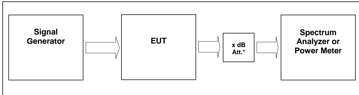
External Attenuator DL x dB = 30 dB figure 5-#1 Test setup: RF Power Out: §24.232, §2.1046
