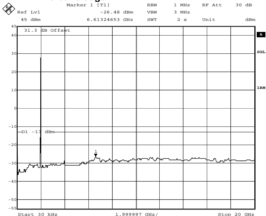
plot 7.3.1.10-#1 Spurious Emissions at Antenna Terminals: §24.238, §2.1051; Test results; Downlink; LTE > 1MHz to band edge; Middle
