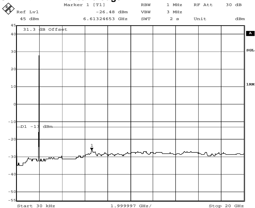
plot 7.3.1.9-#1 Spurious Emissions at Antenna Terminals: §24.238, §2.1051; Test results; Downlink; W-CDMA > 1MHz to band edge; Middle
