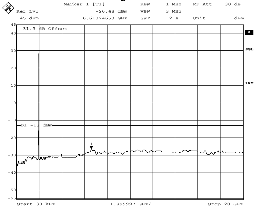
plot 7.3.1.7-#1 Spurious Emissions at Antenna Terminals: §24.238, §2.1051; Test results; Downlink; GSM EDGE > 1MHz to band edge; Middle
