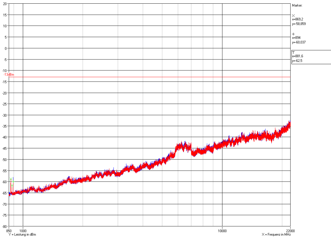
Plot 12.3: Measurement: Field Strength Emission >1 GHz to 22GHz @3m in the FAC max.hold
