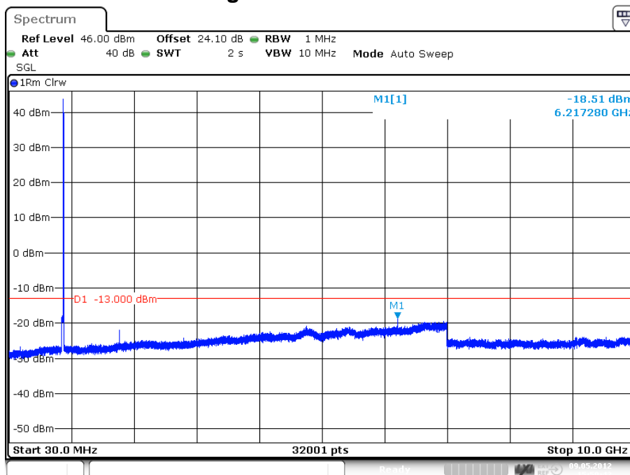
plot 7.3.1.12-#1 Spurious Emissions at Antenna Terminals: §22.917, §2.1051; RSS-131, RSS-GEN; Test results; Downlink; LTE > 1MHz to band edge; carrier (881,5MHz) notched
