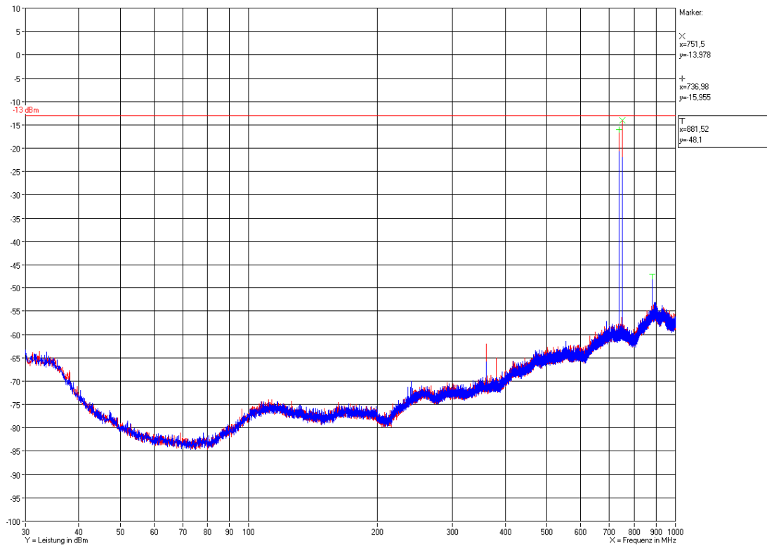
Plot 12.2: Measurement: Field Strength Emission <1 GHz @3m in the FAC max.hold
