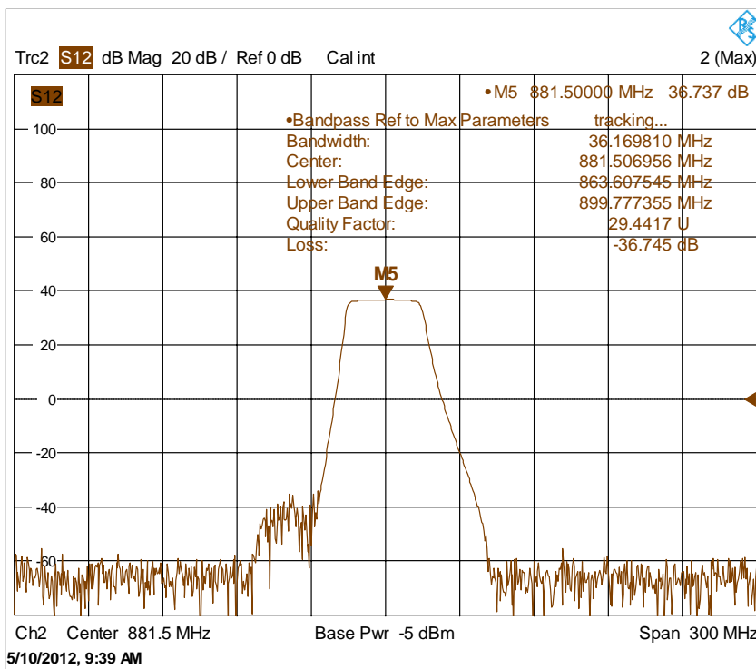
plot 8.3.1-#1 Amplifier Gain and Bandwidth: IC RSS-131; Test results; Downlink
