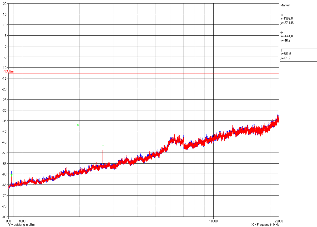
Plot 12.4: Measurement: Field Strength Emission >1 GHz to 22GHz @3m in the FAC max.hold
