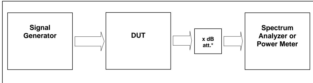
External Attenuator DL x dB = 20 dB figure 6-#1 Test setup: Occupied Bandwidth: §2.1049; RSS-GEN
