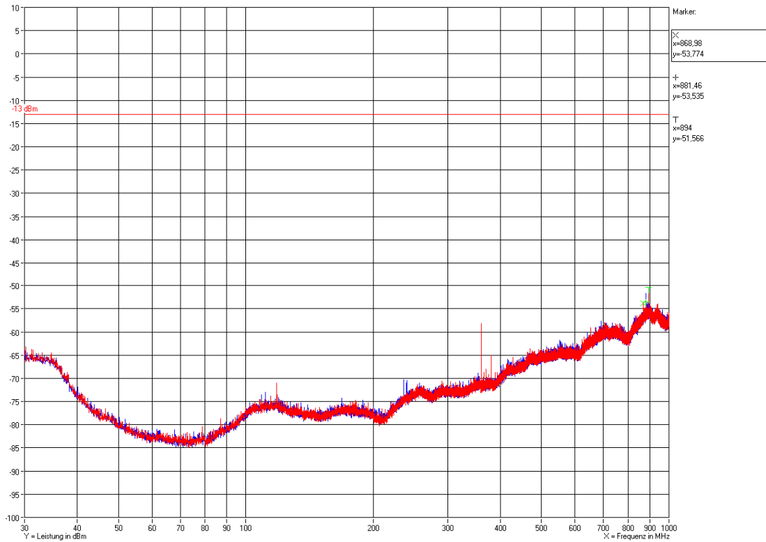
Plot 12.1: Measurement: Field Strength Emission <1 GHz @3m in the FAC max.hold
