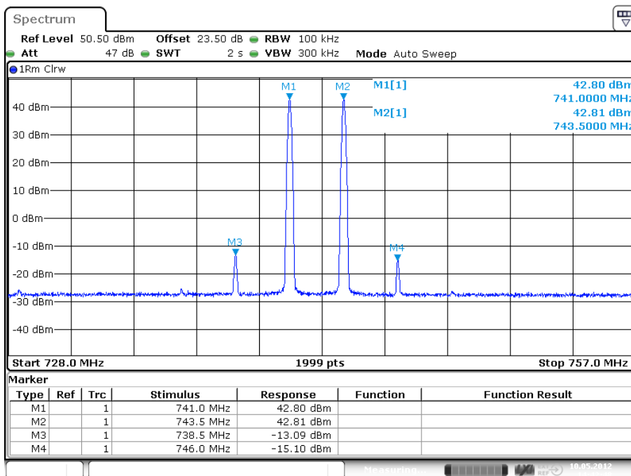
plot 11.3.1-#2 Spurious Emissions: RSS-131; Test results; Downlink; 728 MHz – 757 MHz
