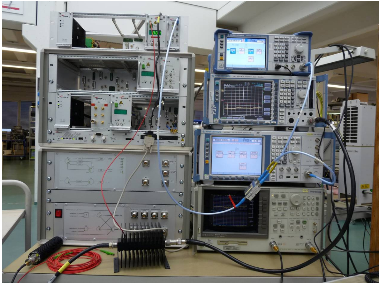
Figure 2. Measurement Equipment
