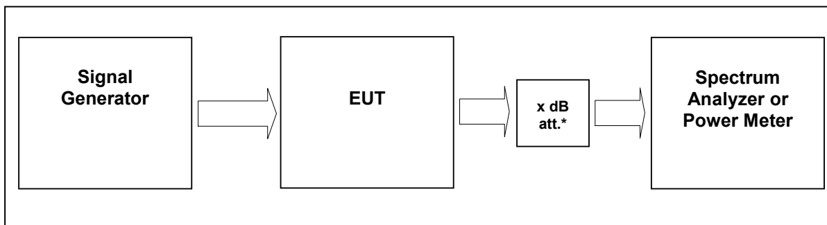
figure 7-#1 Test setup: Spurious Emissions at Antenna Terminals: §27.53, §2.1051
