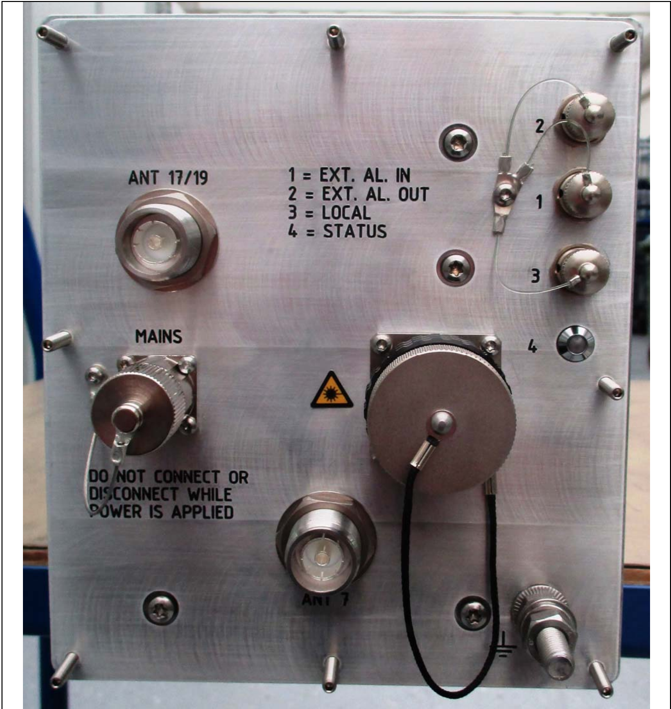
Front Flange
