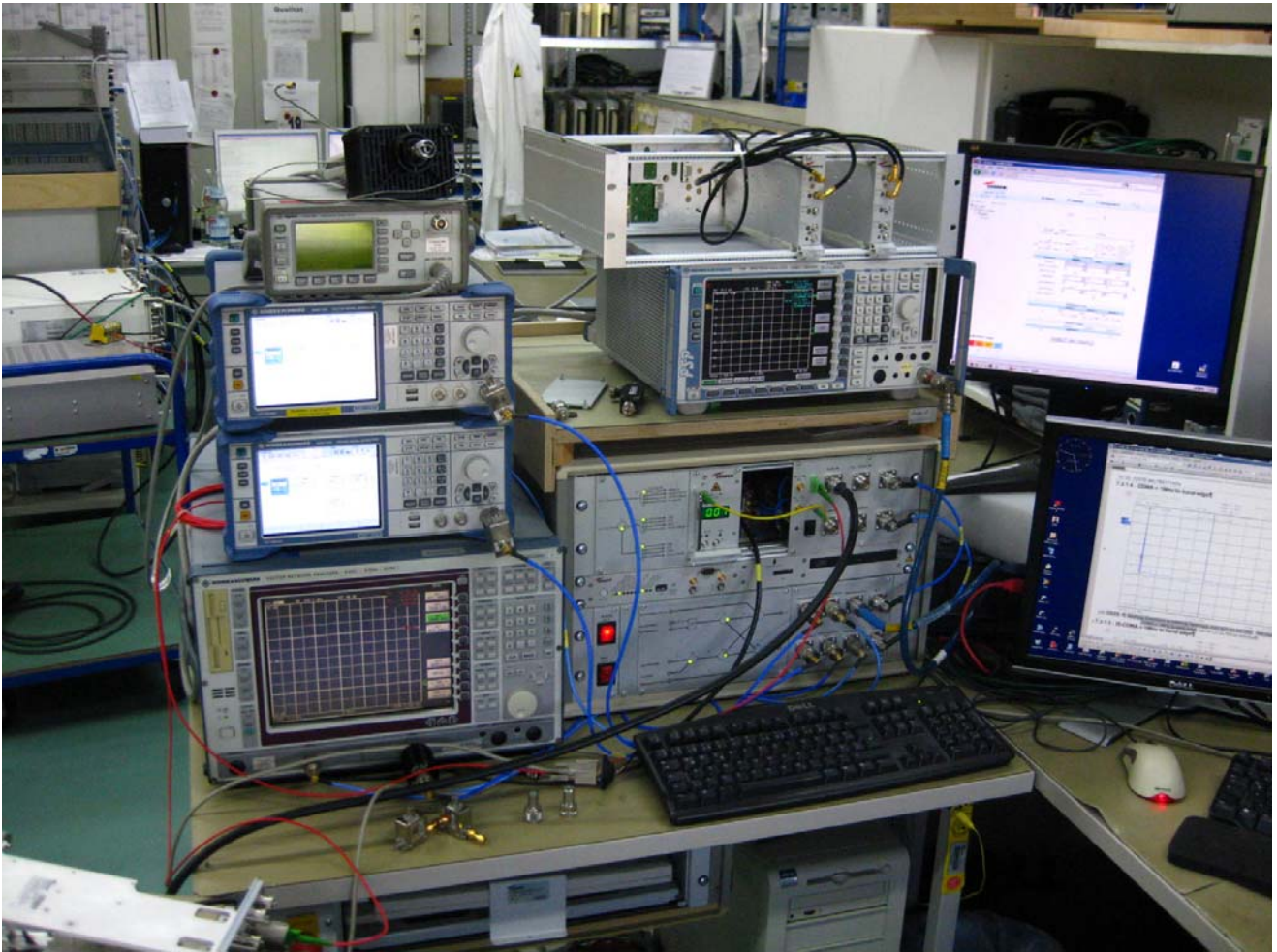
Figure 2. Measurement Equipment
