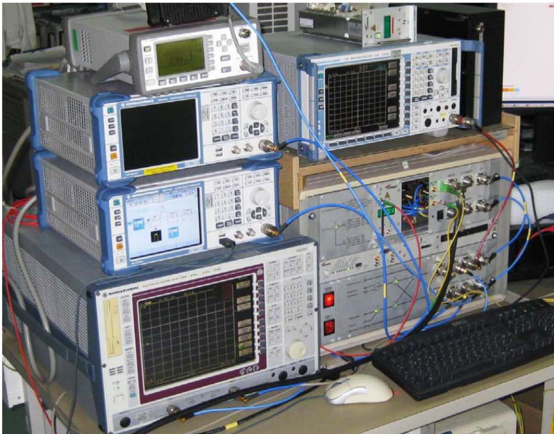
Figure 2. Measurement Equipment
