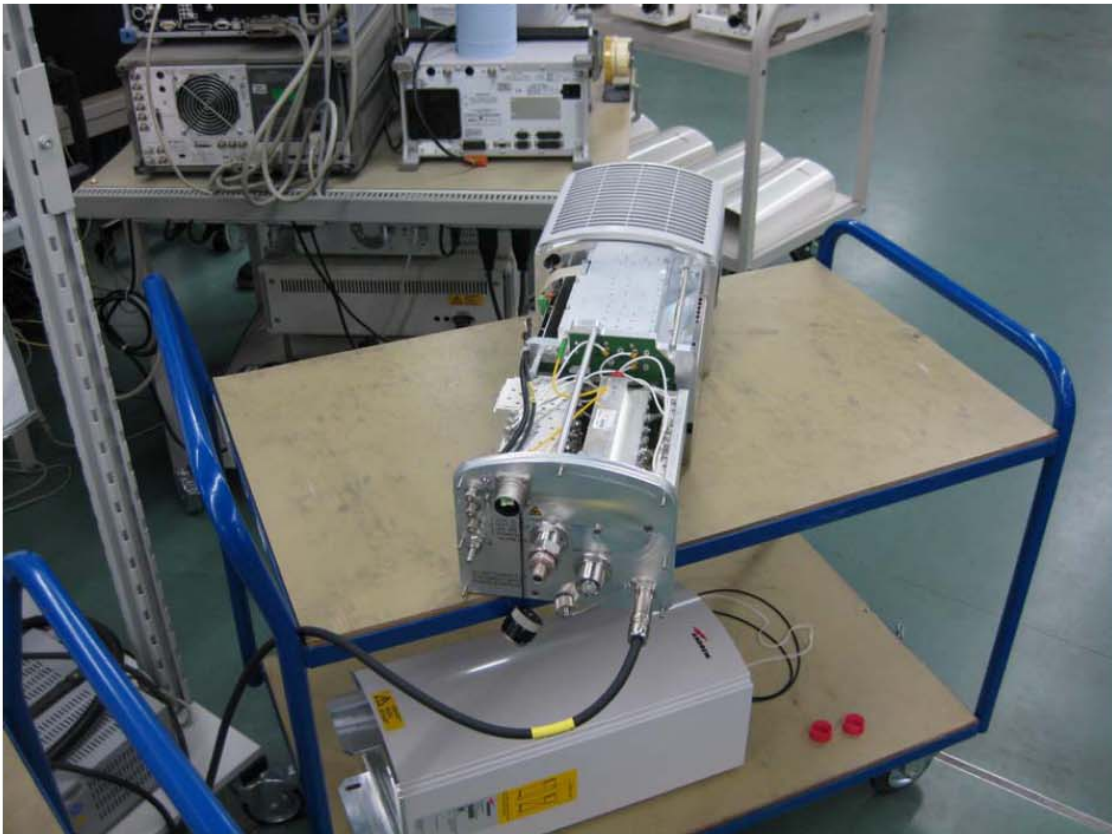
Figure 1. DUT ION-M7P/17P/19P
