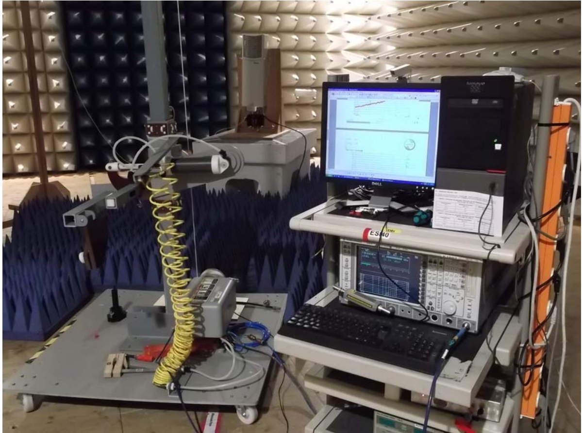
Figure 3. radiated spurious emission
