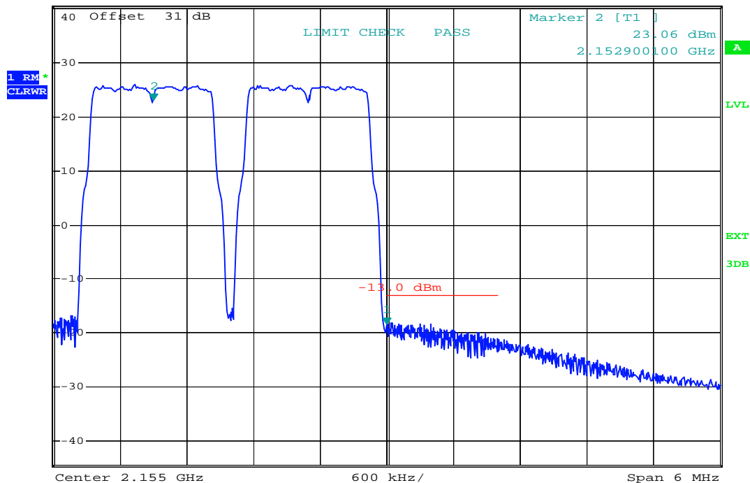
plot 7.3.1.3-#2 Spurious Emissions at Antenna Terminals: §27.53, §2.1051; Test results; Downlink; LTE < 1MHz to band edge Upper Band Edge
