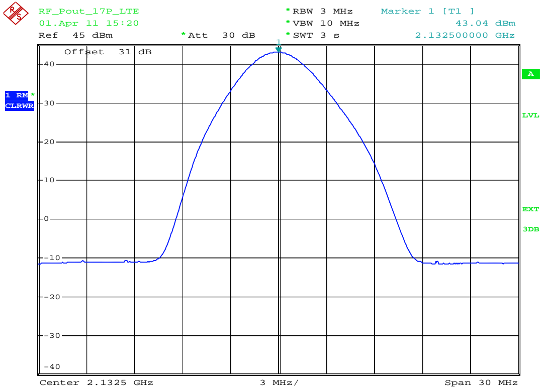
plot 5.3.1.3-#1 RF Power Out: §27.50, §2.1046; Test results; Downlink; LTE Middle
