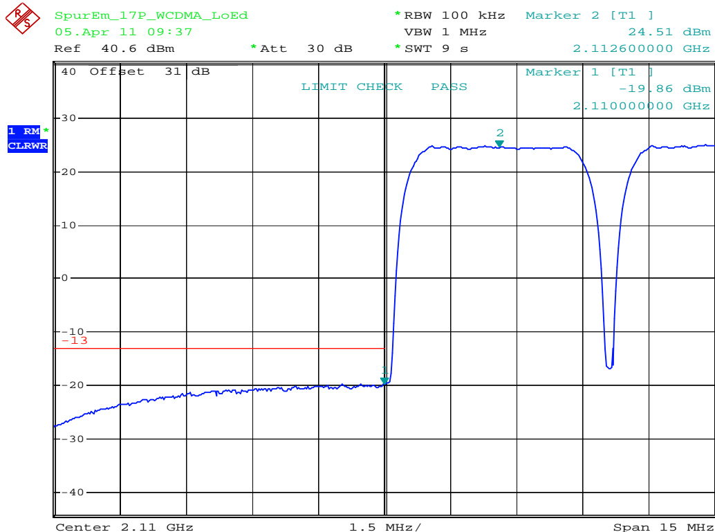
plot 7.3.1.1-#1 Spurious Emissions at Antenna Terminals: §27.53, §2.1051; Test results; Downlink; WCDMA < 1MHz to band edge Lower Band Edge
