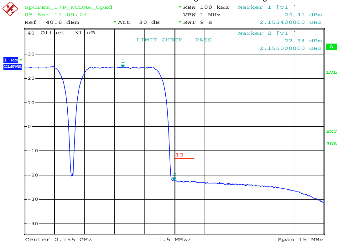
plot 7.3.1.1-#2 Spurious Emissions at Antenna Terminals: §27.53, §2.1051; Test results; Downlink; WCDMA < 1MHz to band edge Upper Band Edge
