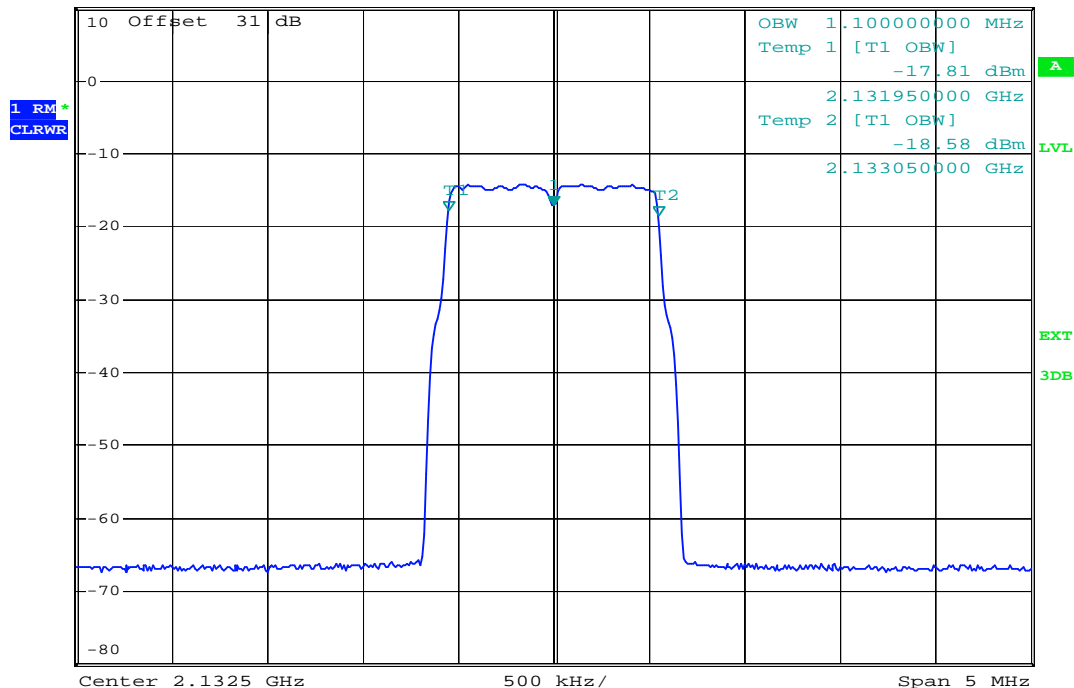
plot 6.3.1.3-#2 Occupied Bandwidth: §2.1049; Test results; Downlink; LTE Input
