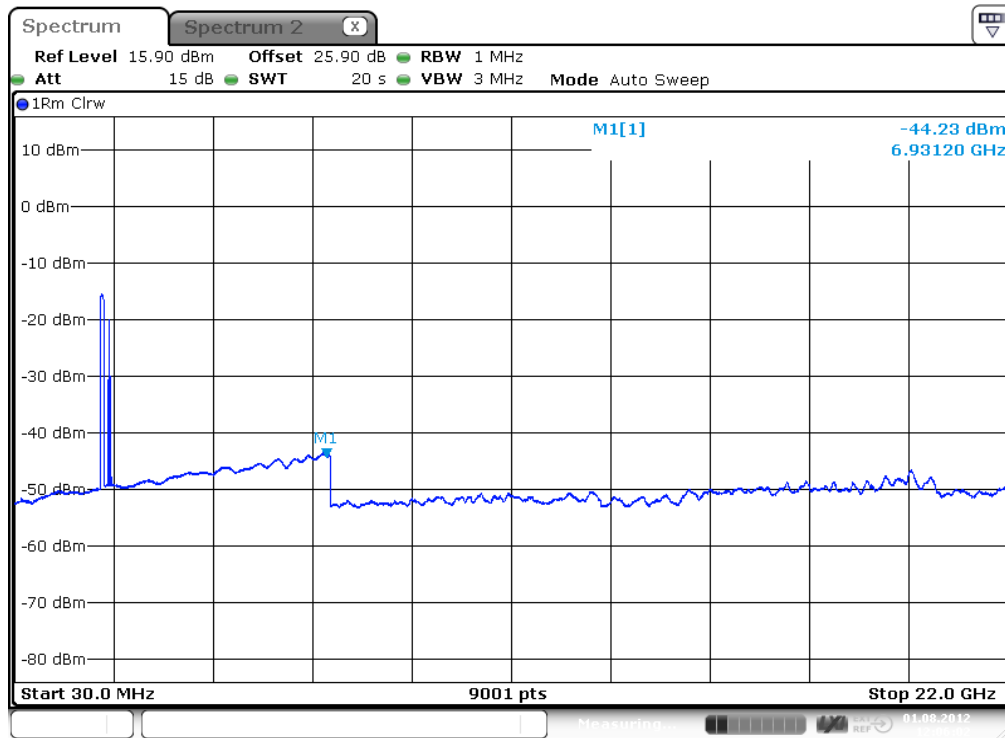
plot 7.3.1.6-#1 Spurious Emissions at Antenna Terminals: §27.53, §2.1051; Test results; Downlink; LTE > 1MHz to band edge; carrier (2132,5MHz) notched
