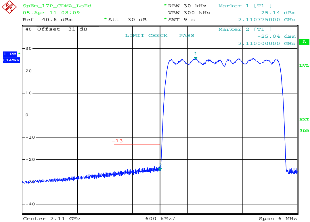
plot 7.3.1.2-#1 Spurious Emissions at Antenna Terminals: §27.53, §2.1051; Test results; Downlink; CDMA < 1MHz to band edge Lower Band Edge
