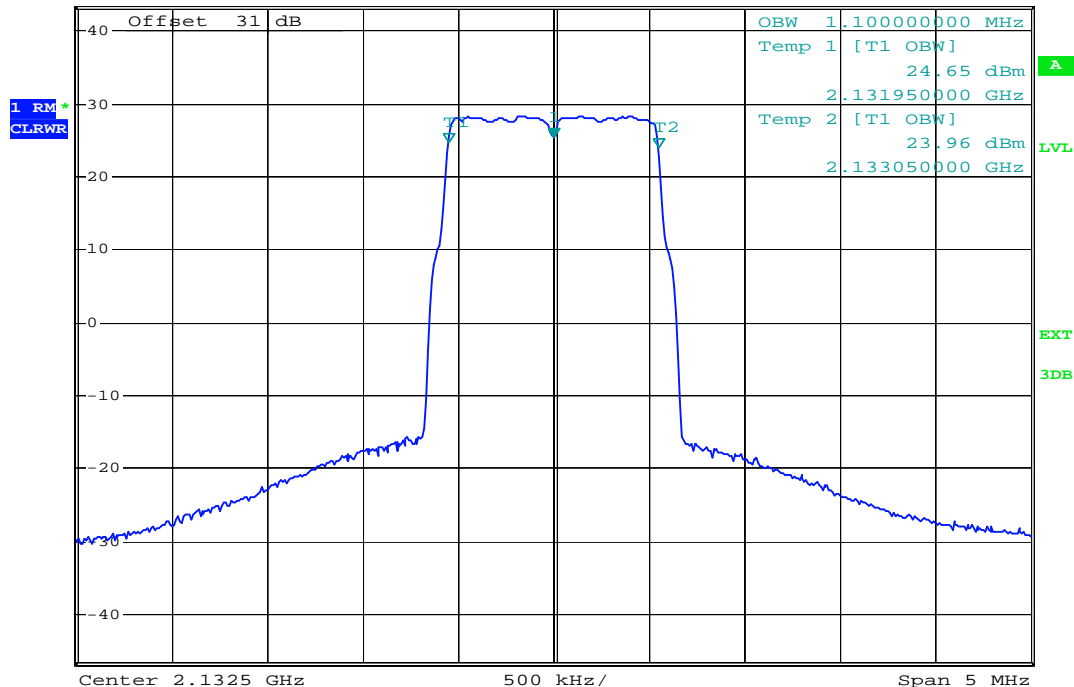
plot 6.3.1.3-#1 Occupied Bandwidth: §2.1049; Test results; Downlink; LTE Output
