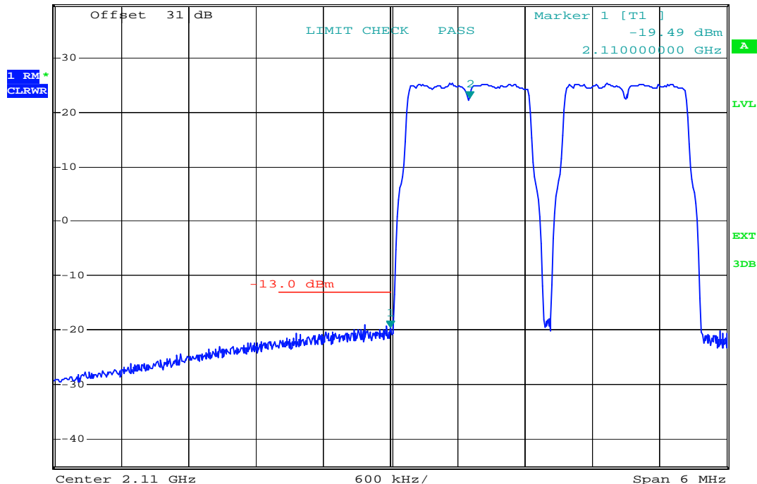
plot 7.3.1.3-#1 Spurious Emissions at Antenna Terminals: §27.53, §2.1051; Test results; Downlink; LTE < 1MHz to band edge Lower Band Edge
