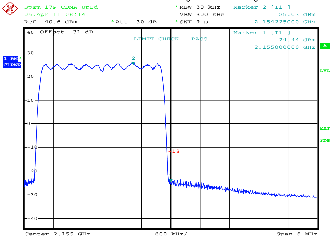
plot 7.3.1.2-#2 Spurious Emissions at Antenna Terminals: §27.53, §2.1051; Test results; Downlink; CDMA < 1MHz to band edge Upper Band Edge
