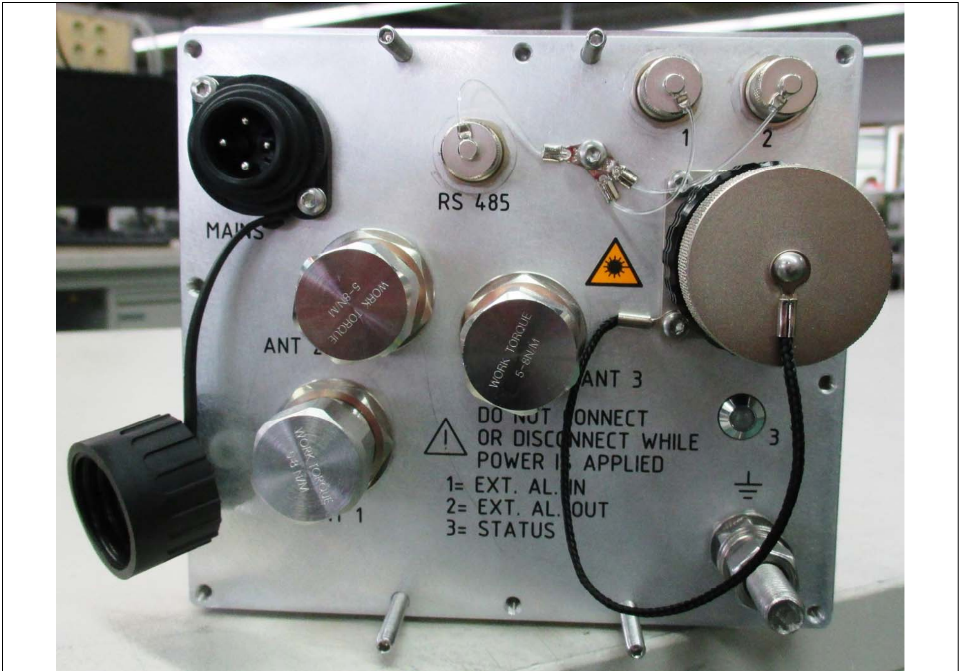
Front Flange
