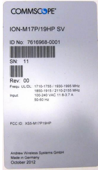
picture 8.1: Name plate
