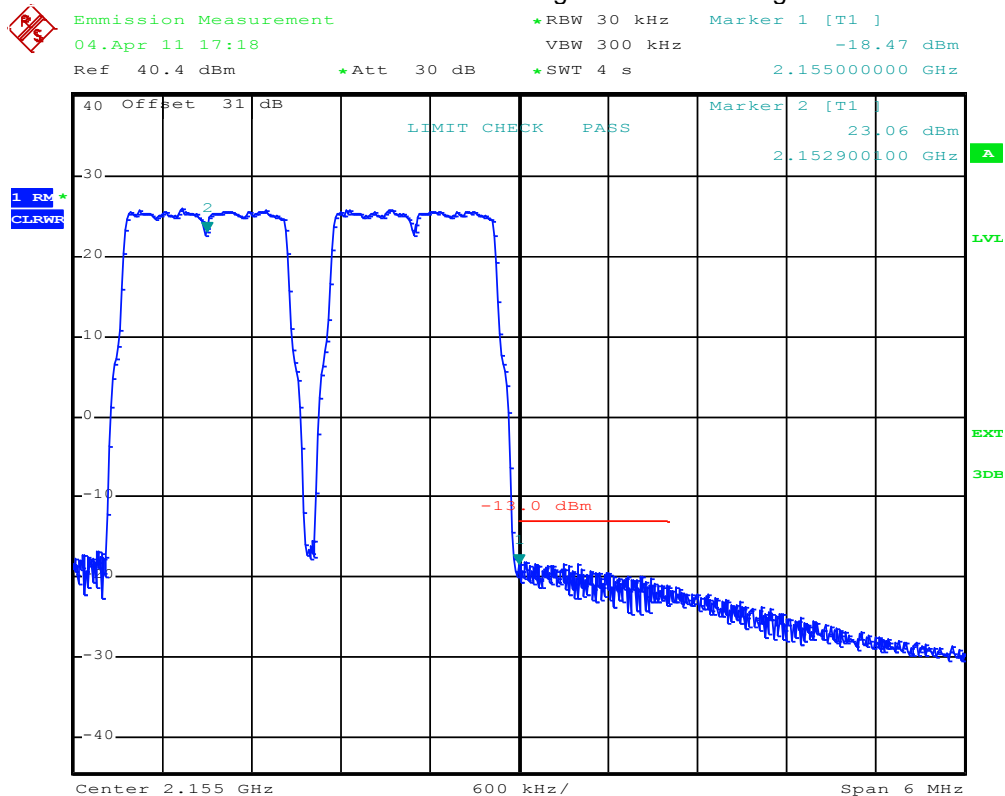
plot 7.3.1.3-#2 Spurious Emissions at Antenna Terminals: FCC §27.53, §2.1051; Test results; Downlink; LTE < 1MHz to band edge Upper Band Edge
