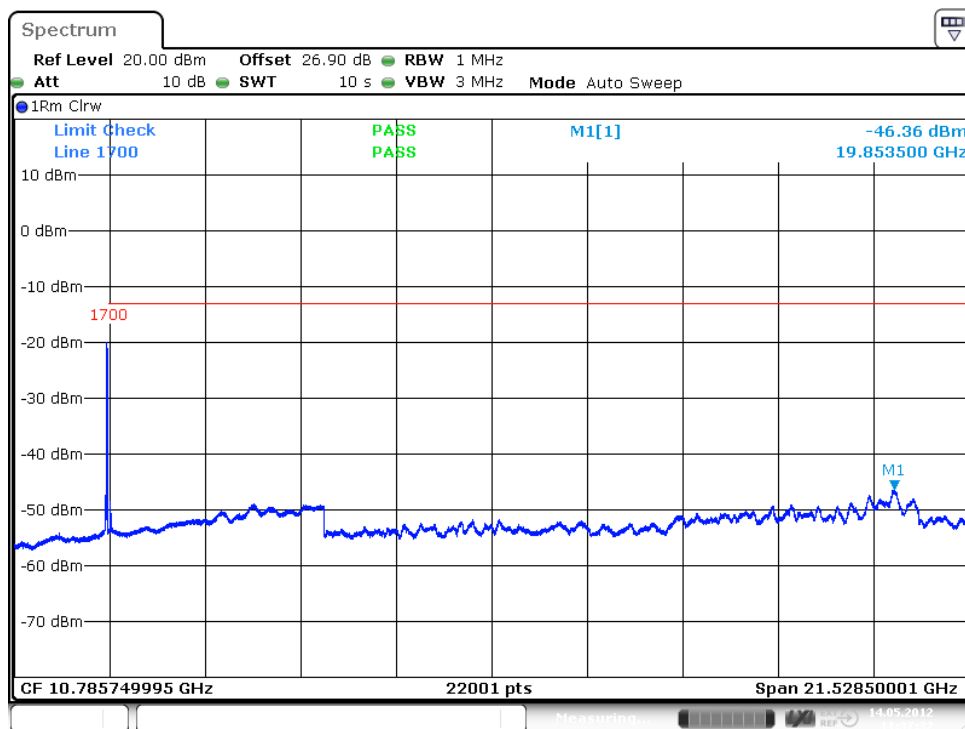
plot 7.3.1.6-#1 Spurious Emissions at Antenna Terminals: FCC §27.53, §2.1051; Test results; Downlink; LTE > 1MHz to band edge; carrier (2132,5MHz) notched
