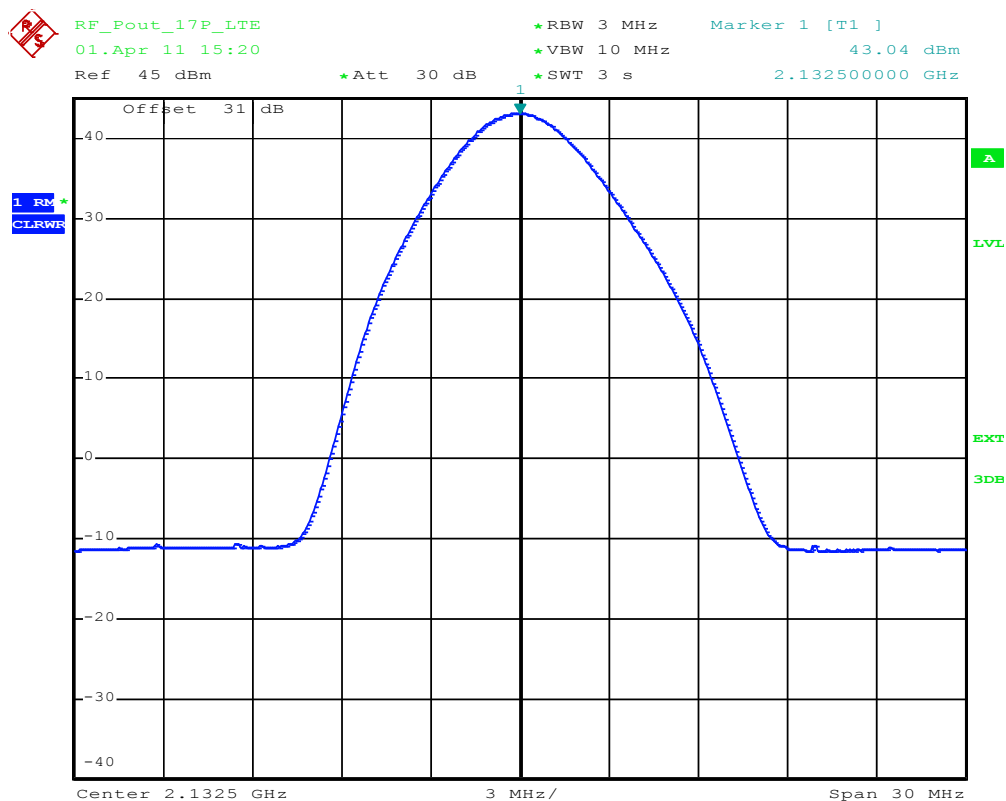
plot 5.3.1.3-#1 RF Power Out: FCC §27.50, §2.1046; Test results; Downlink; LTE Middle
