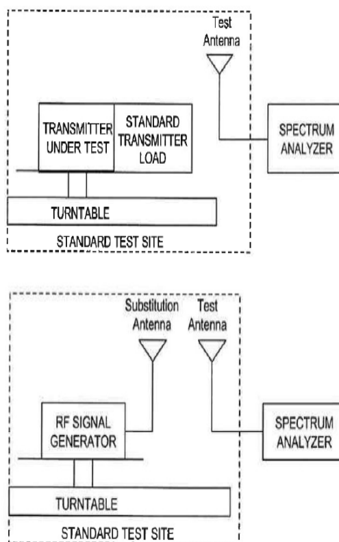
Figure #7.2 Substitution methods TIA/EIA-603-C
