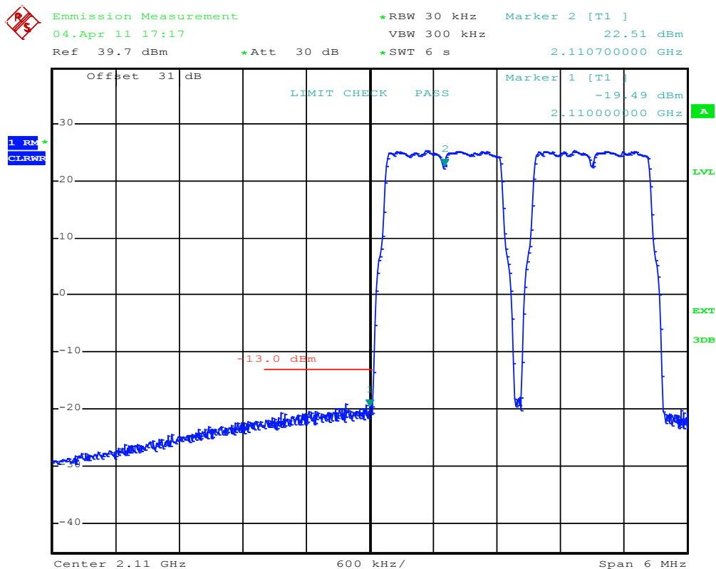
plot 7.3.1.3-#1 Spurious Emissions at Antenna Terminals: FCC §27.53, §2.1051; Test results; Downlink; LTE < 1MHz to band edge Lower Band Edge
