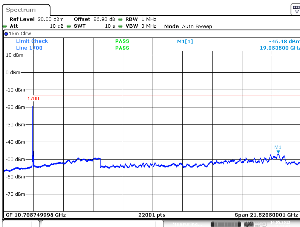
plot 7.3.1.5-#1 Spurious Emissions at Antenna Terminals: FCC §27.53, §2.1051; Test results; Downlink; W-CDMA > 1MHz to band edge; carrier (2132,5MHz) notched
