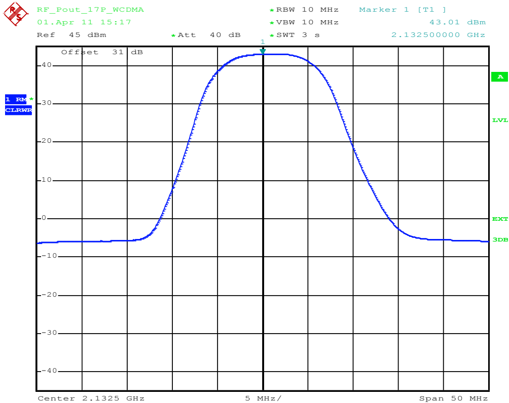
plot 5.3.1.2-#1 RF Power Out: FCC §27.50, §2.1046; Test results; Downlink; W-CDMA Middle
