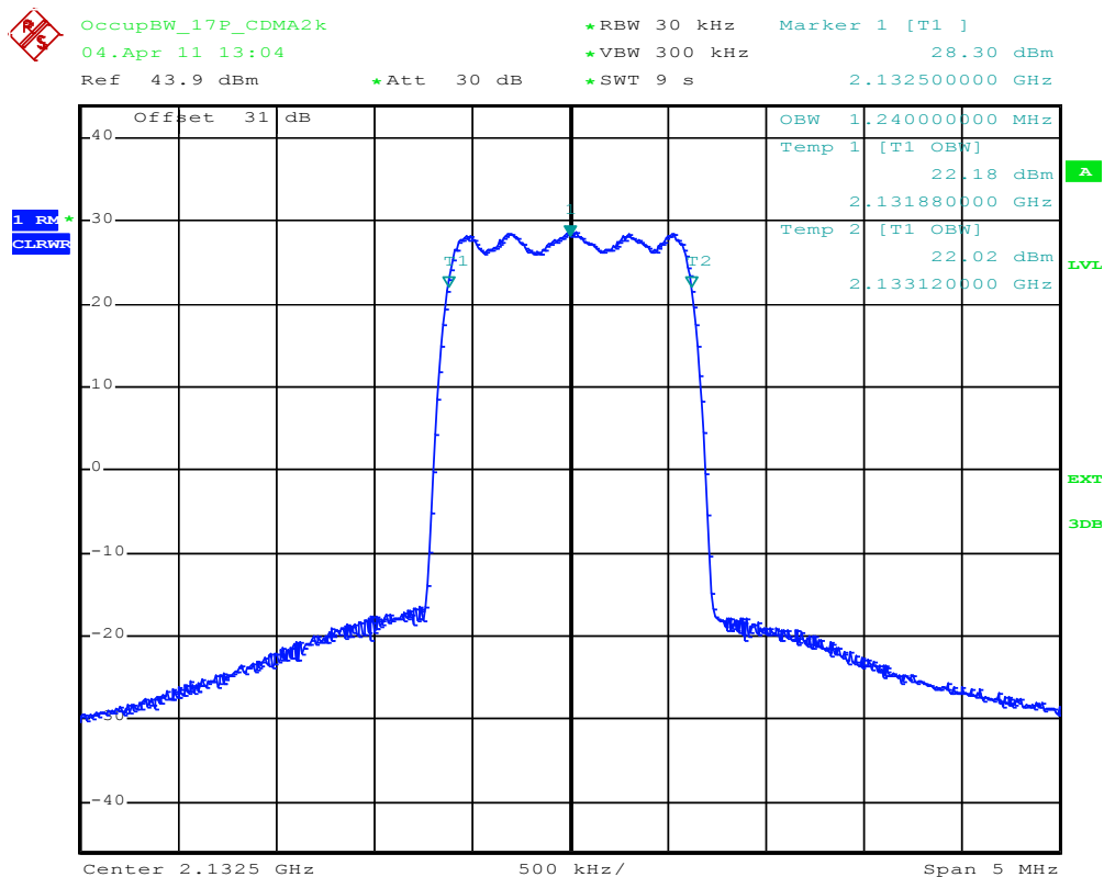
plot 6.3.1.1-#1 Occupied Bandwidth: FCC §2.1049; RSS-GEN; Test results; Downlink; CDMA Output
