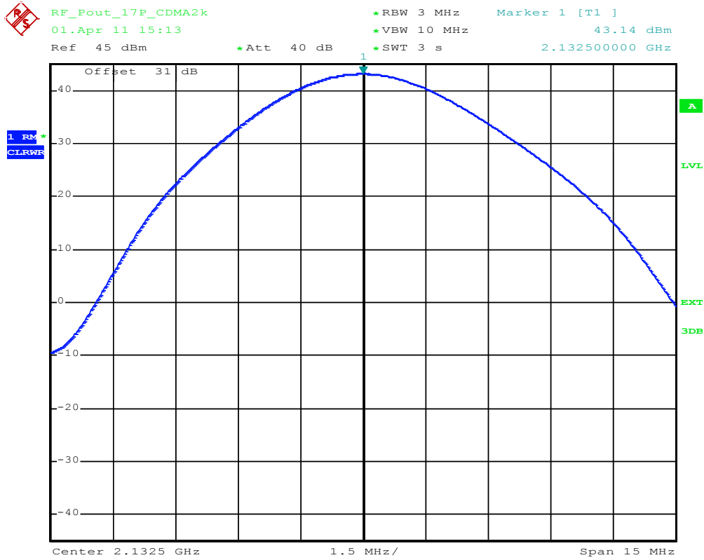
plot 5.3.1.1-#1 RF Power Out: FCC §27.50, §2.1046; Test results; Downlink; CDMA Middle
