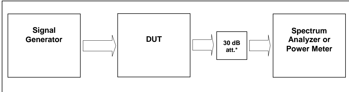
figure 5.4-#1 Test setup: Occupied Bandwidth: FCC §2.1049; RSS-GEN
