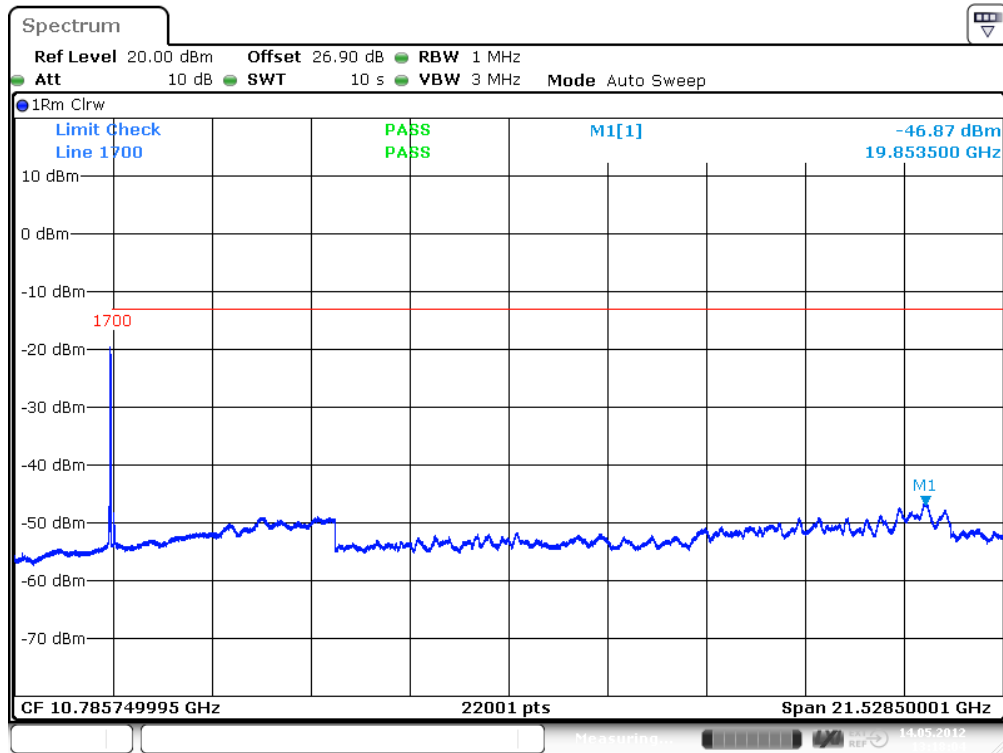
plot 7.3.1.4-#1 Spurious Emissions at Antenna Terminals: FCC §27.53, §2.1051; Test results; Downlink; CDMA > 1MHz to band edge; carrier (2132,5MHz) notched
