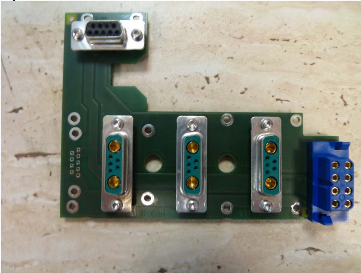
Duplexer PCB 7580558-01
