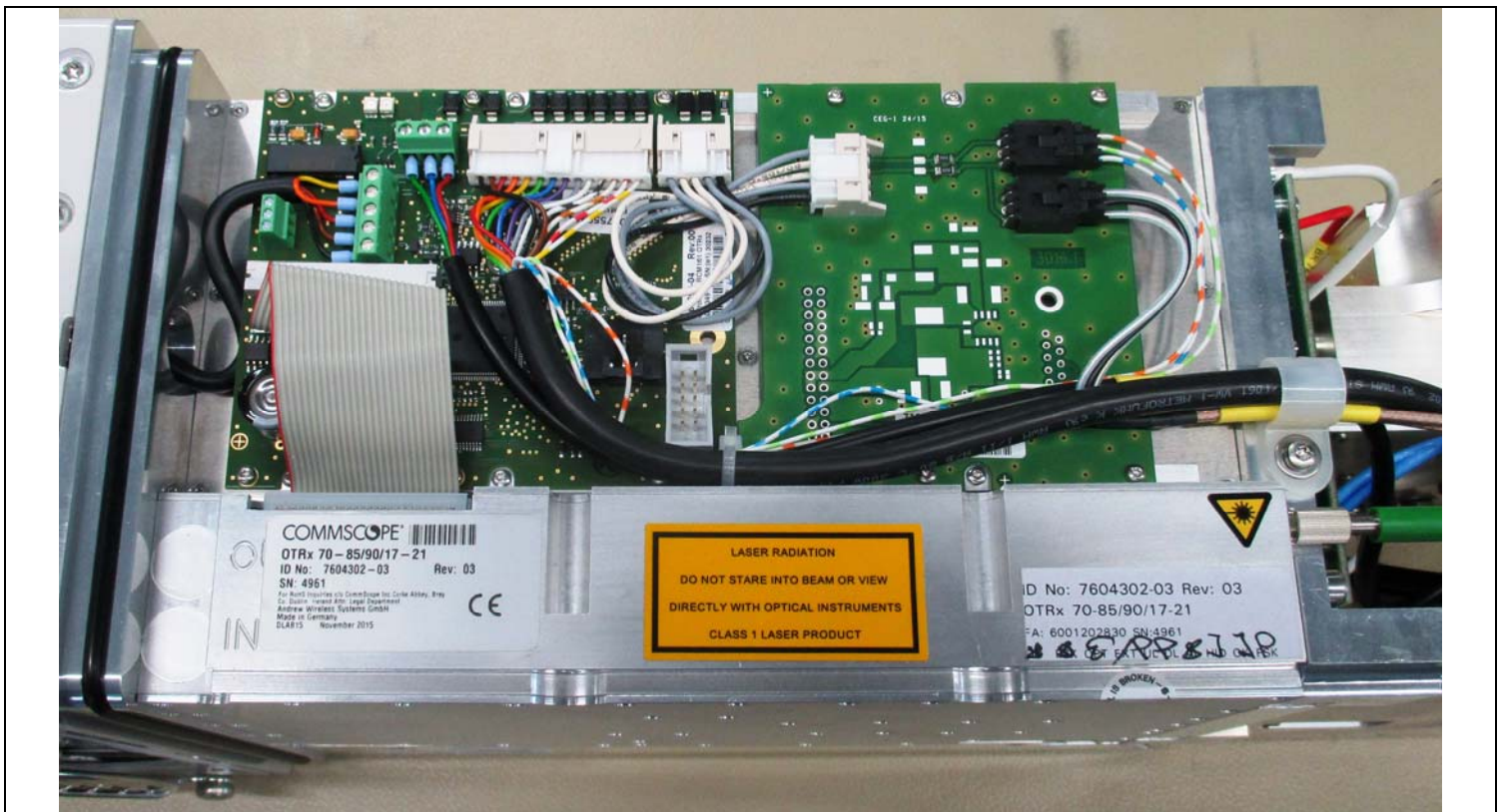
Controller PCB
