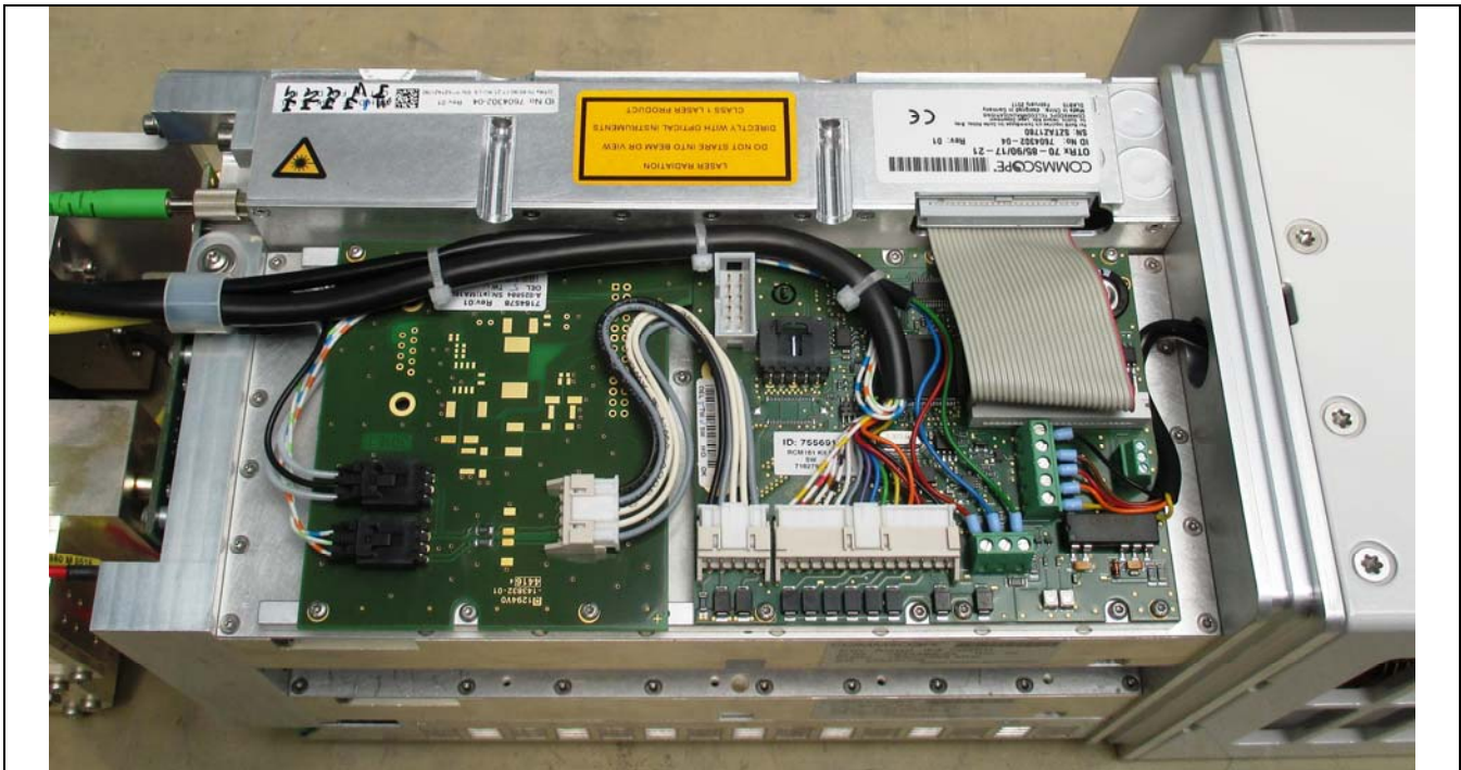
Controller PCB
