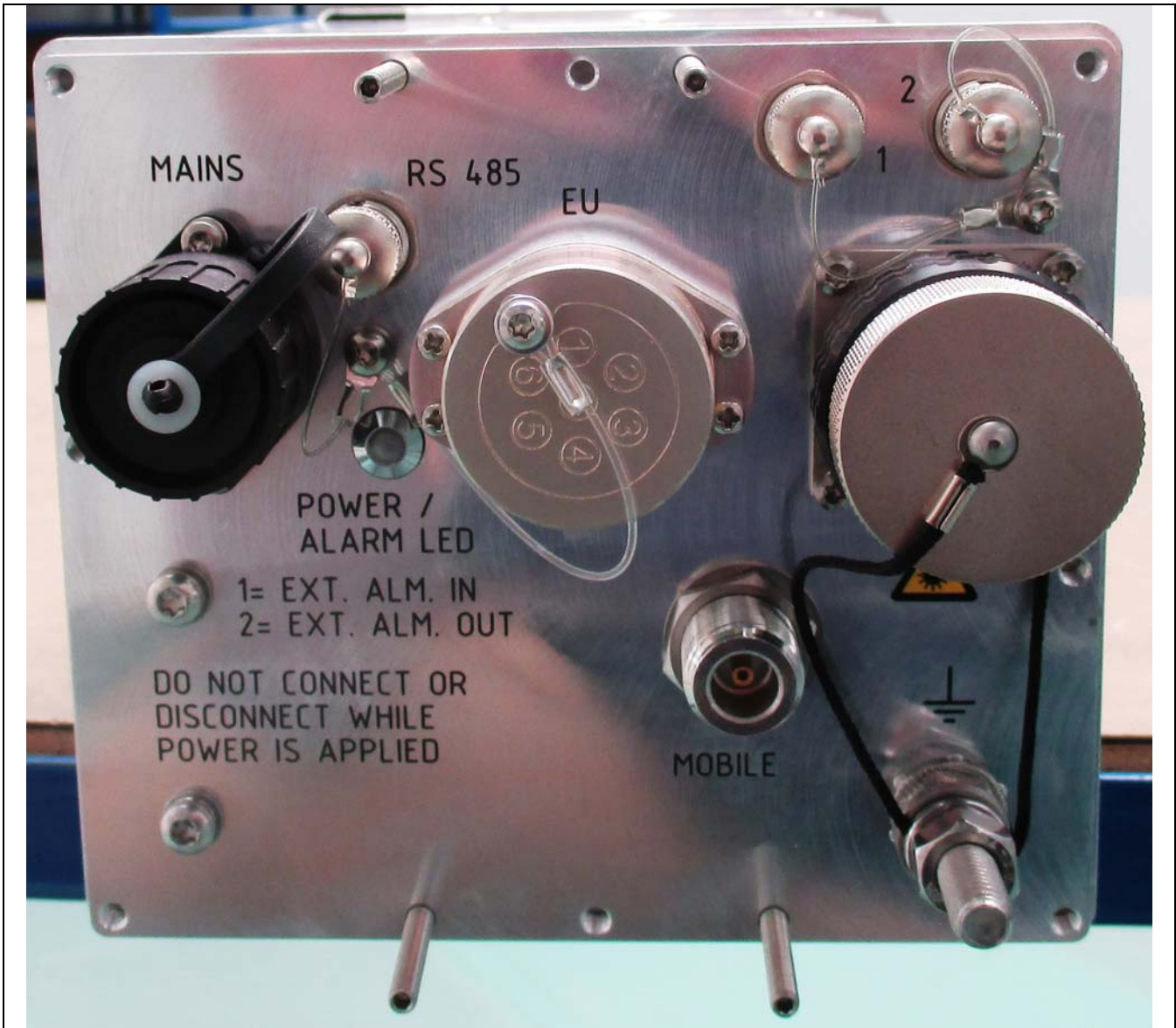
Front Flange
