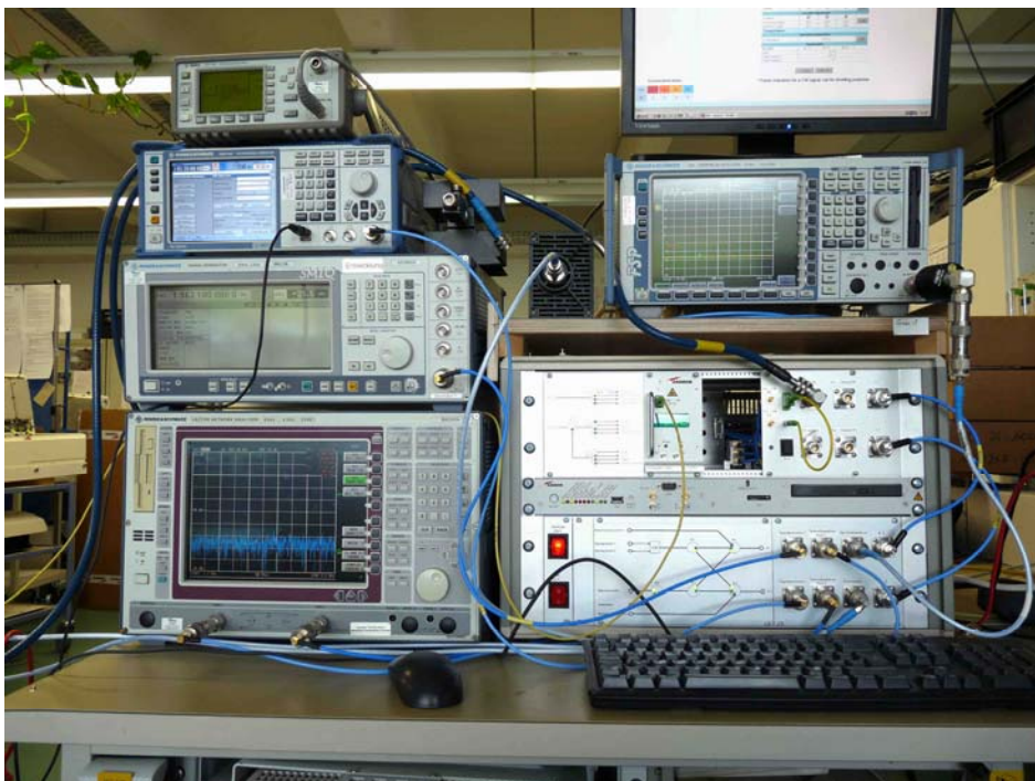
Figure 2. Measurement Equipment
