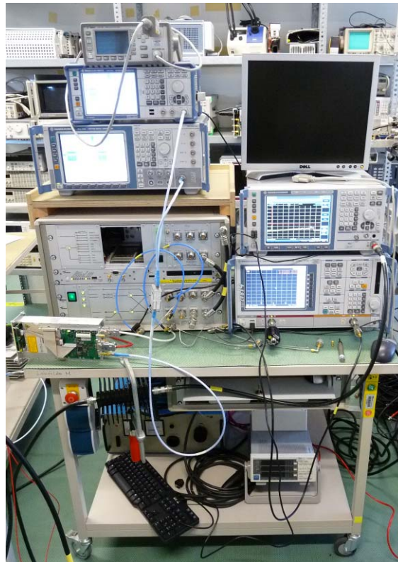
Figure 2. Measurement Equipment
