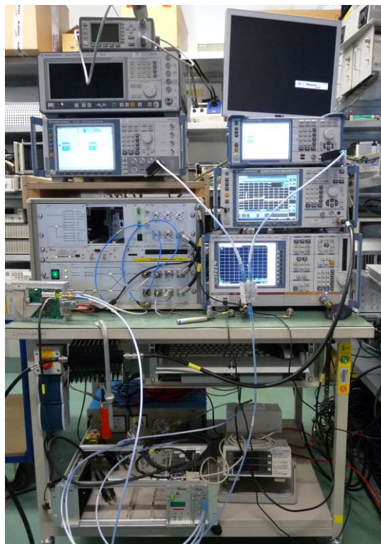
Figure 2. Measurement Equipment
