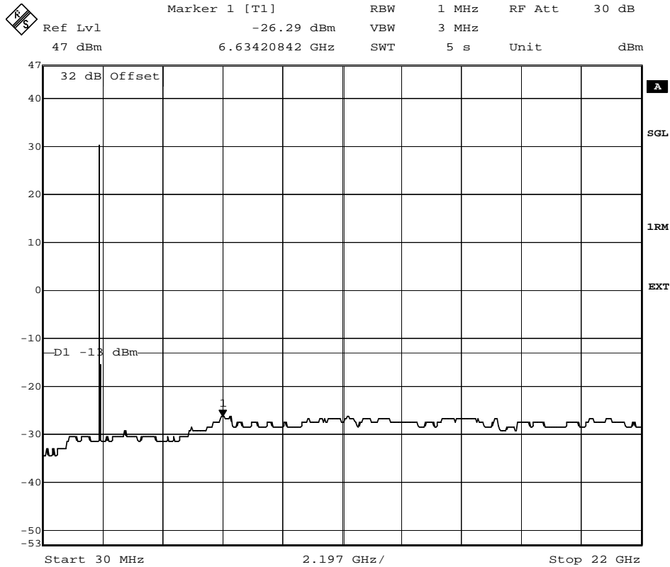
plot 7.3.1.5-#1 Spurious Emissions at Antenna Terminals: §27.53, §2.1051; Test results; Downlink; W-CDMA > 1MHz to band edge; carrier (2132,5MHz) notched
