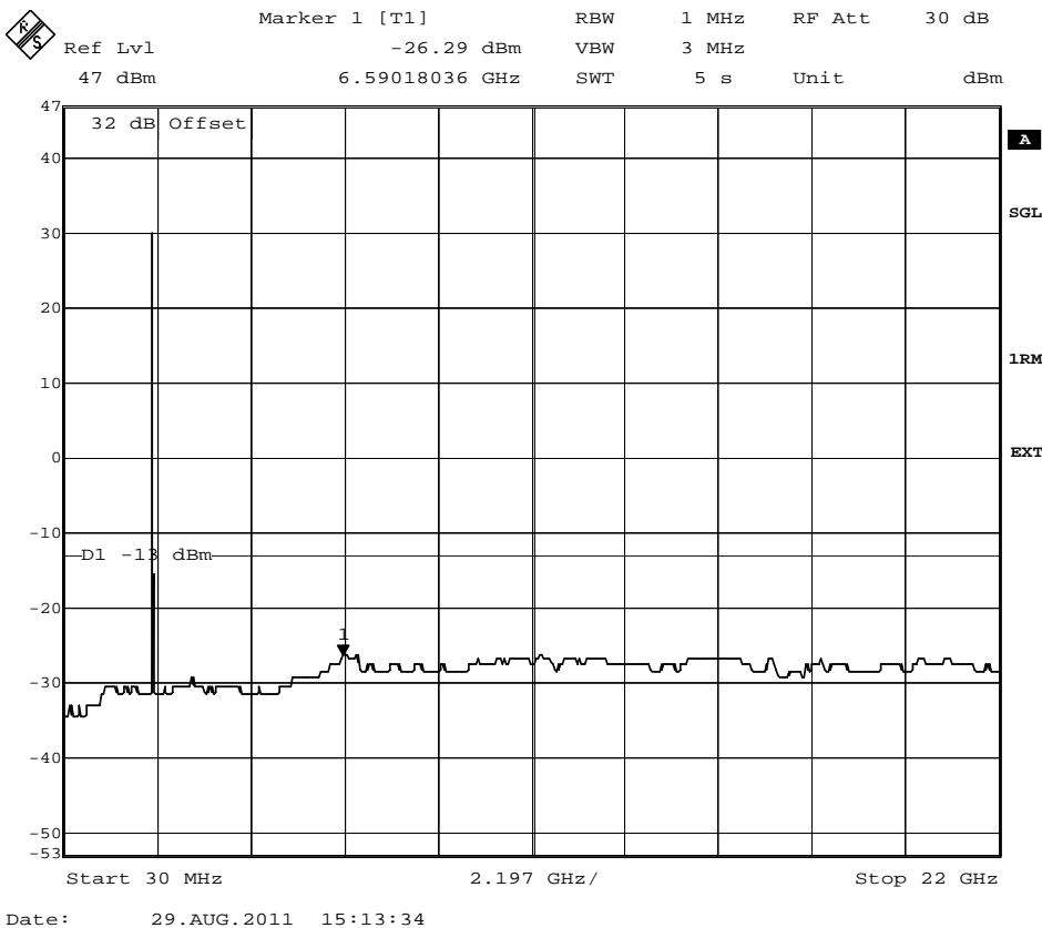
plot 7.3.1.6-#1 Spurious Emissions at Antenna Terminals: §27.53, §2.1051; Test results; Downlink; LTE > 1MHz to band edge; carrier (2132,5MHz) notched
