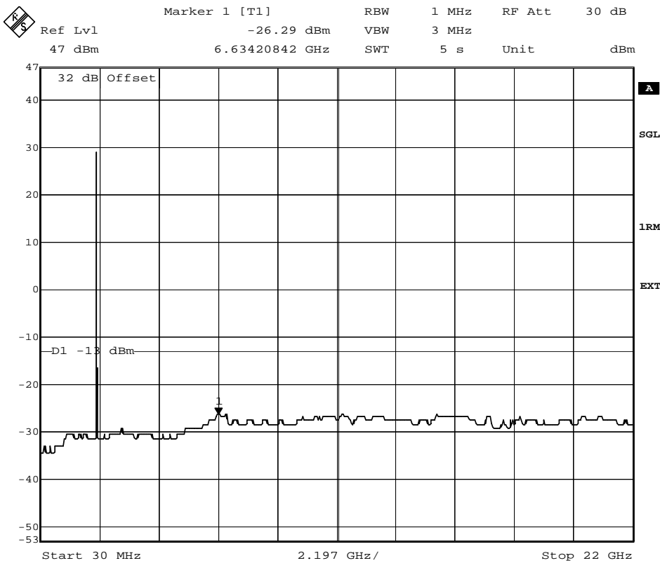
plot 7.3.1.4-#1 Spurious Emissions at Antenna Terminals: §27.53, §2.1051; Test results; Downlink; CDMA > 1MHz to band edge; carrier (2132,5MHz) notched
