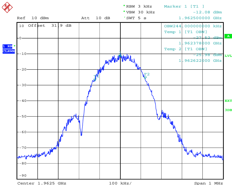
plot 6.3.1.2-#1 Occupied Bandwidth: §2.1049; Test results; Downlink; GSM-EDGE Output
