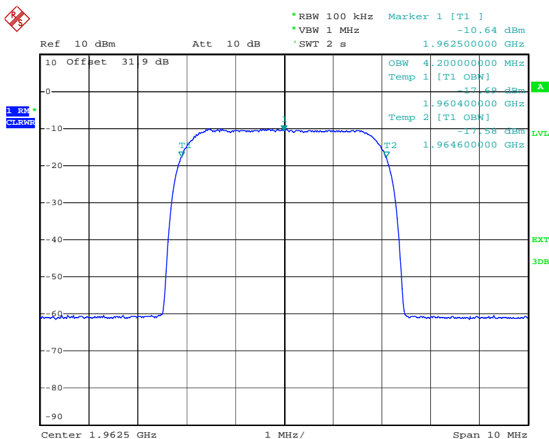
plot 6.3.1.4-#1 Occupied Bandwidth: §2.1049; Test results; Downlink; W-CDMA Output
