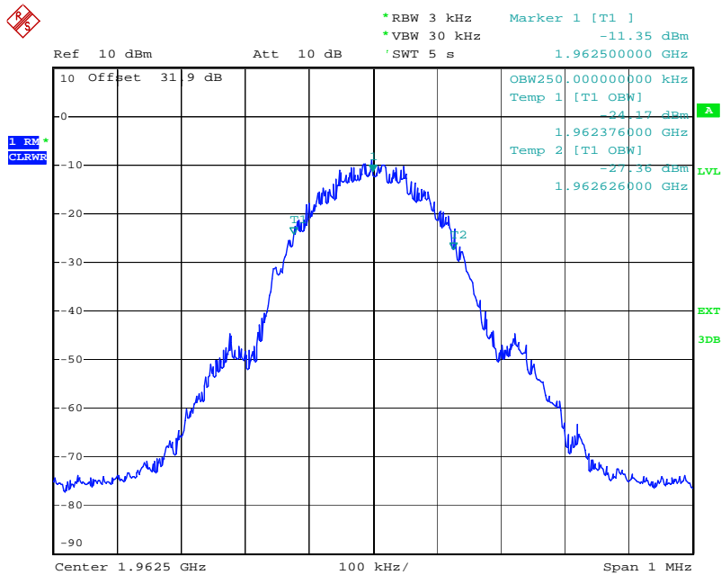
plot 6.3.1.1-#1 Occupied Bandwidth: §2.1049; Test results; Downlink; GSM Output
