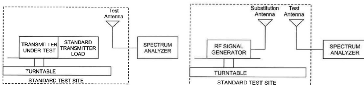
picture 8.3: Substitution method
