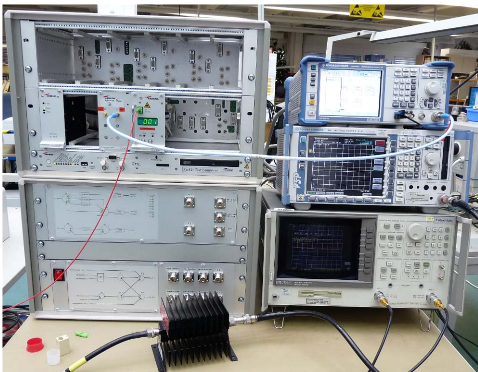
Figure 2. Measurement Equipment
