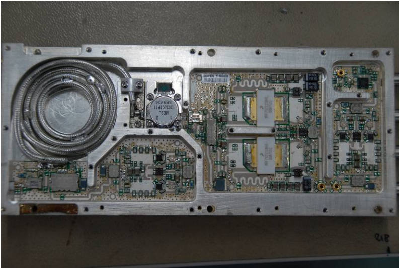
Amplifier bottom:
