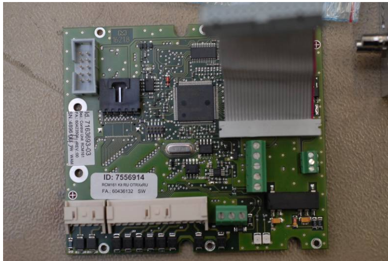
Controller top:
