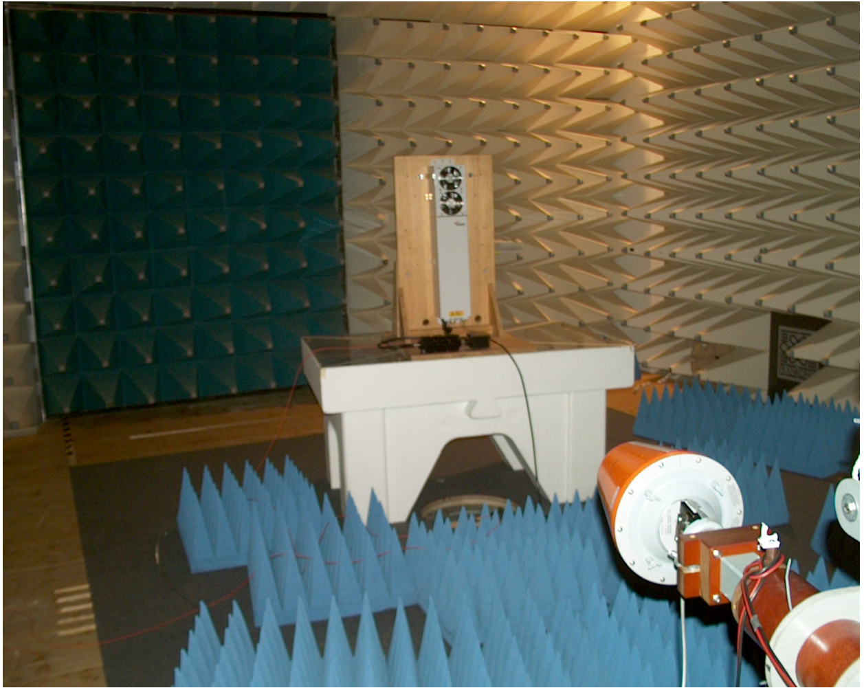
Test set-up for radiated spurious emission >1GHz @3m in the FAC
