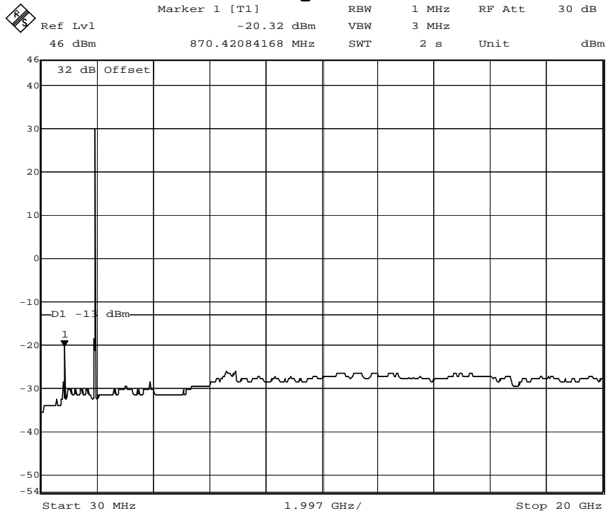
plot 7.3.1.7-#1 Spurious Emissions at Antenna Terminals: §24.238, §2.1051; Test results; Downlink; GSM EDGE > 1MHz to band edge; Middle
