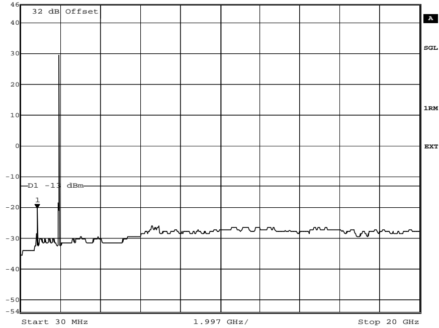
plot 7.3.1.10-#1 Spurious Emissions at Antenna Terminals: §24.238, §2.1051; Test results; Downlink; LTE > 1MHz to band edge; Middle
