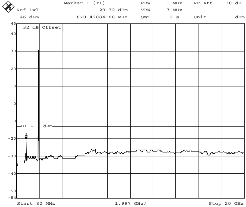
plot 7.3.1.6-#1 Spurious Emissions at Antenna Terminals: §24.238, §2.1051; Test results; Downlink; GSM > 1MHz to band edge; Middle
