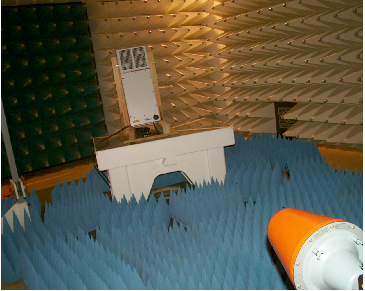
picture 1: Test setup: Field Strength Emission 1GHz to 20GHz @3m in the FAC
