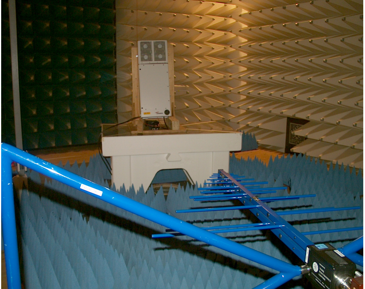
picture 2: Test setup: Field Strength Emission <1 GHz @3m in the FAC
