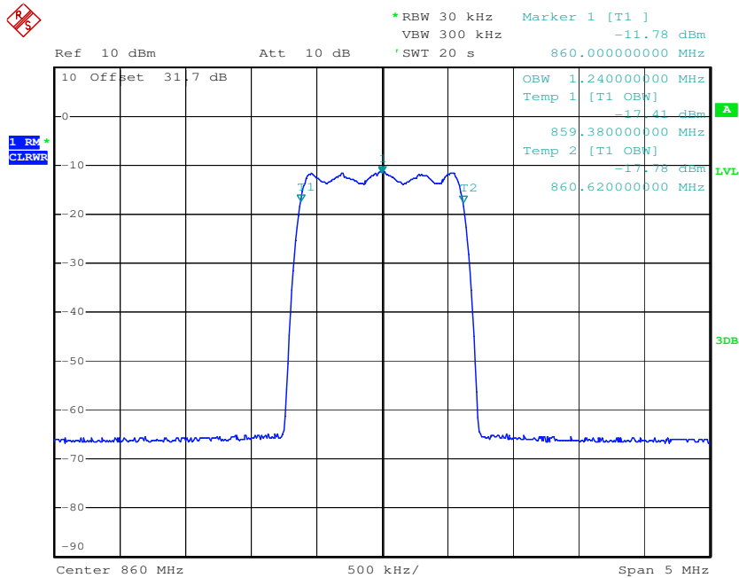
plot 6.3.1.5-#1 Occupied Bandwidth: §90.210, §2.1049; RSS-GEN; Test results; Downlink; EV-DO Output
