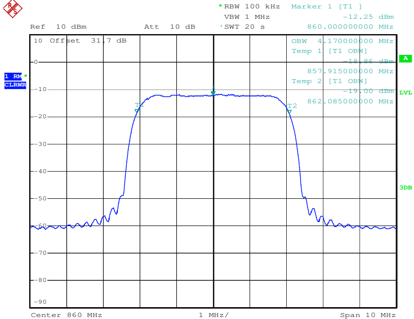
plot 6.3.1.7-#1 Occupied Bandwidth: §90.210, §2.1049; RSS-GEN; Test results; Downlink; HSPA Output
