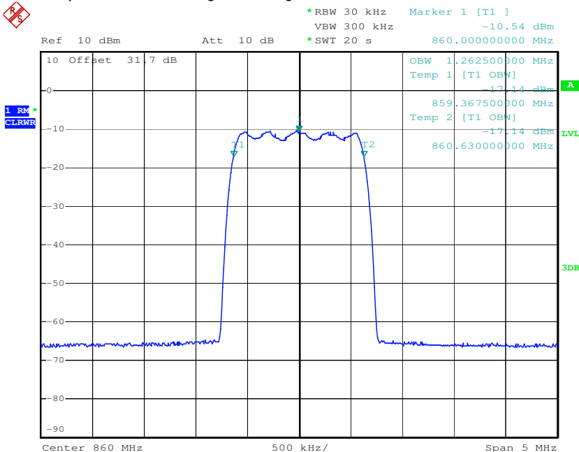
plot 6.3.1.4-#1 Occupied Bandwidth: §90.210, §2.1049; RSS-GEN; Test results; Downlink; CDMA Output
