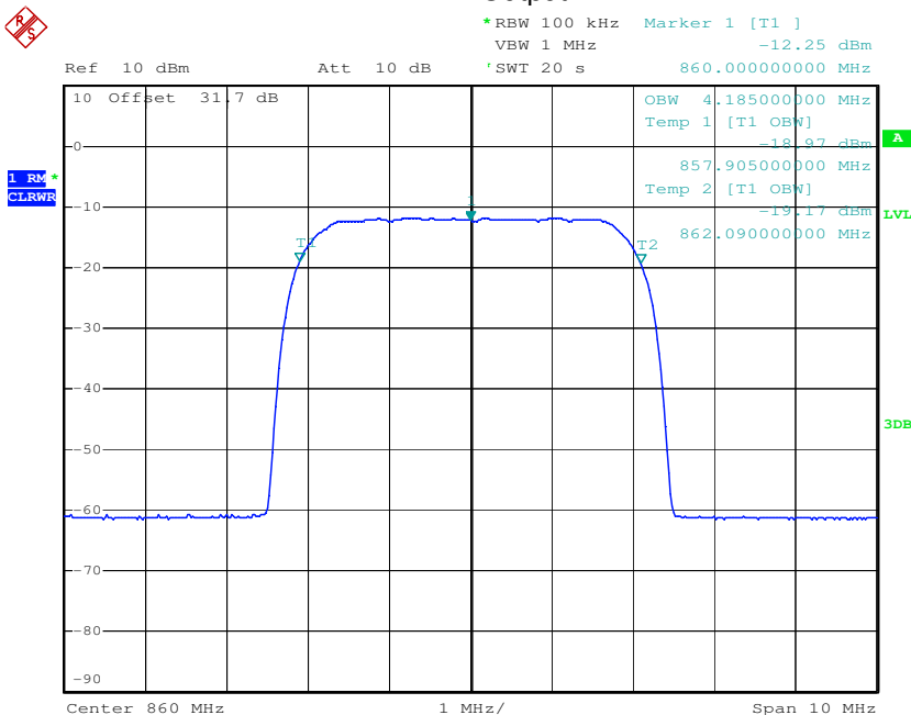
plot 6.3.1.6-#1 Occupied Bandwidth: §90.210, §2.1049; RSS-GEN; Test results; Downlink; WCDMA Output
