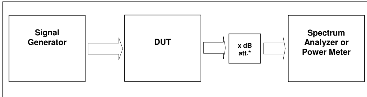
External Attenuator DL x dB = 30 dB figure 6-#1 Test setup: Occupied Bandwidth: §90.210, §2.1049; RSS-GEN
