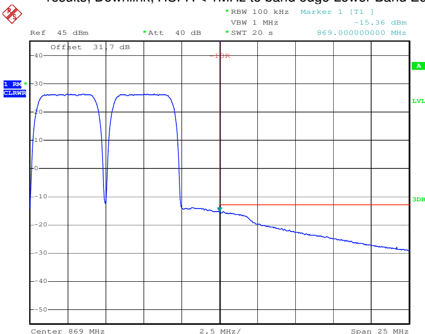
plot 7.3.1.7-#1 Spurious Emissions at Antenna Terminals: §90.210, §2.1051; RSS-131, RSS-GEN; Test results; Downlink; HSPA < 1MHz to band edge Lower Band Edge
