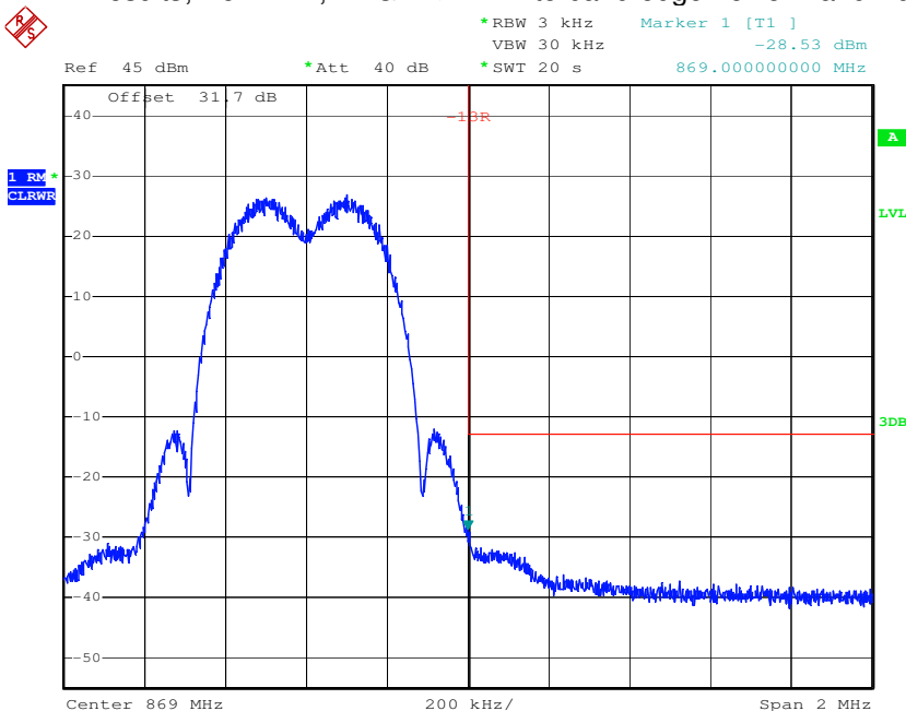
plot 7.3.1.3-#1 Spurious Emissions at Antenna Terminals: §90.210, §2.1051; RSS-131, RSS-GEN; Test results; Downlink; EDGE < 1MHz to band edge Lower Band Edge
