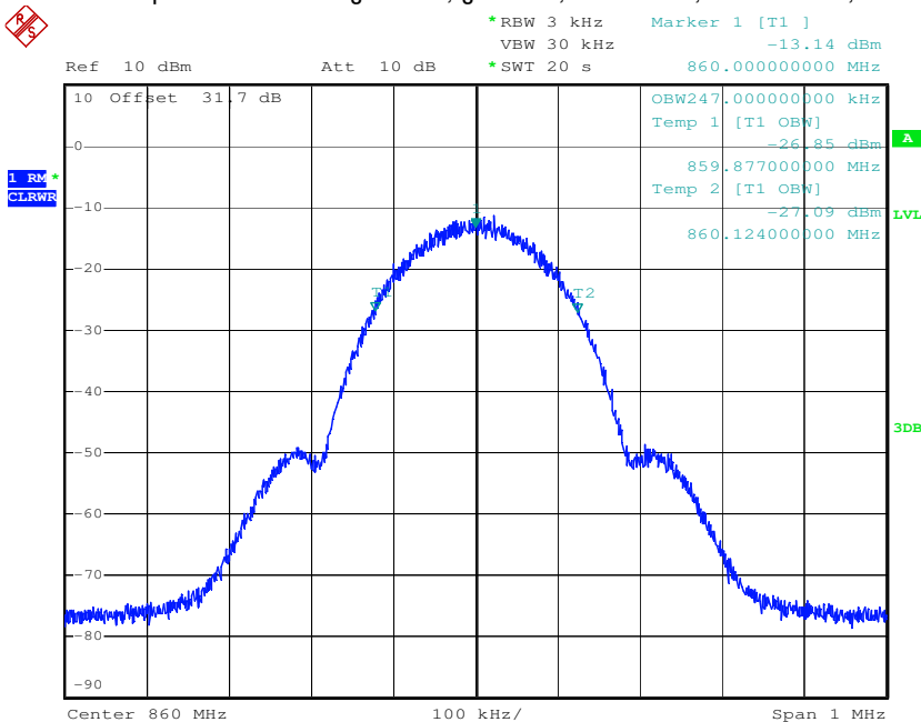
plot 6.3.1.2-#1 Occupied Bandwidth: §90.210, §2.1049; RSS-GEN; Test results; Downlink; TDMA Output
