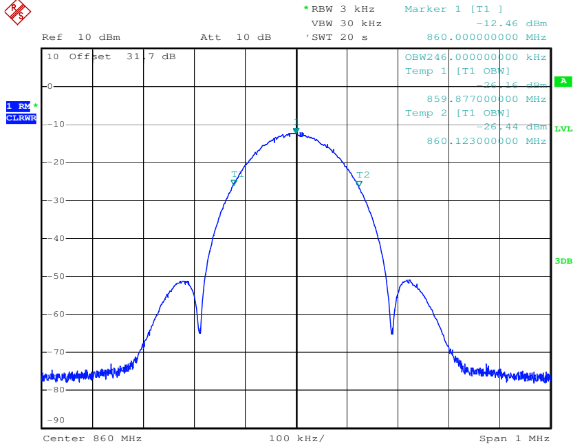
plot 6.3.1.3-#1 Occupied Bandwidth: §90.210, §2.1049; RSS-GEN; Test results; Downlink; EDGE Output
