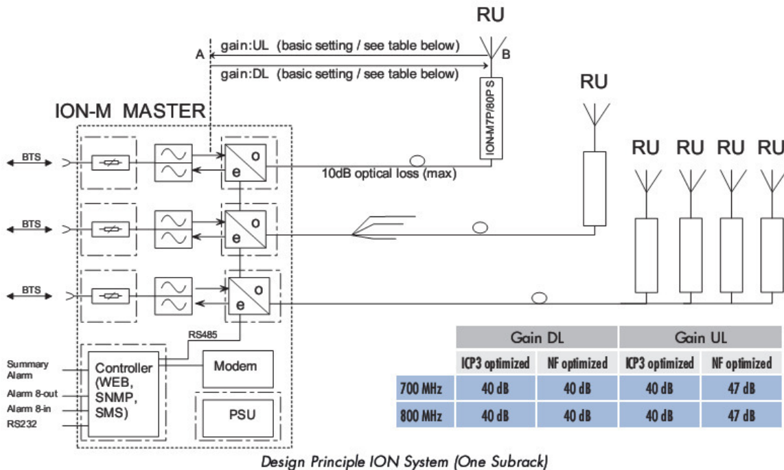
figure 2.1.4-#2 System diagrams: EUT is Remote Unit
