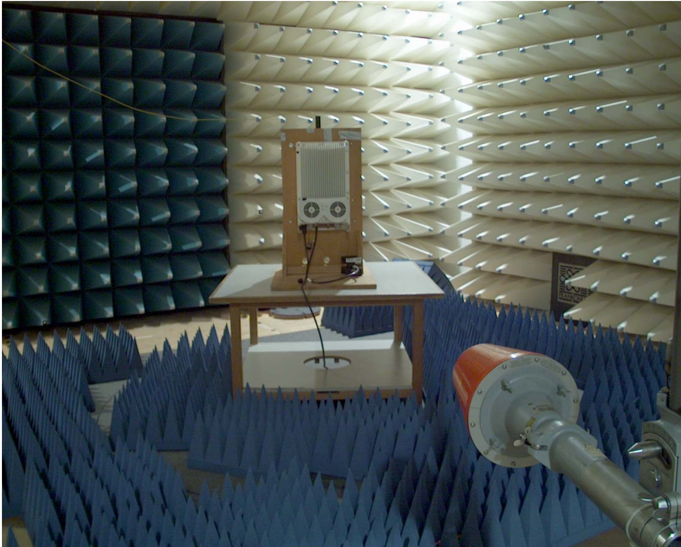
Test setup >1 GHz @3m distance
