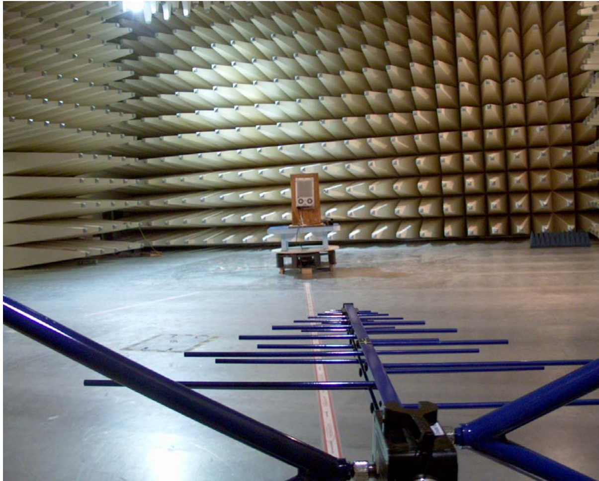
Test setup <1 GHz @ 10m distance
